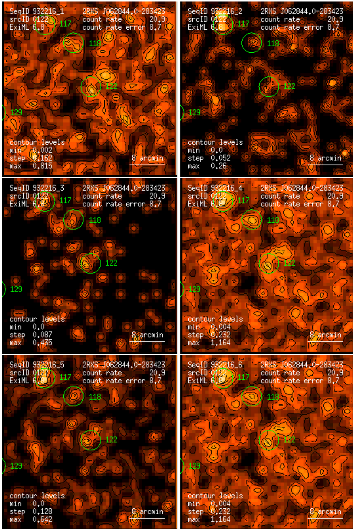
Figure 122: RASS 932216: detection 0122: band rate images, Gaussian filter: (1) PSPC channels 11 – 41, (2) 52 – 90, (3) 91 – 201, (4) 11 – 235, (5) 52 – 201, (6) 11 – 201. Broad band rates in counts/ks. Band rate contour levels in counts/ks/arcmin 2 .
