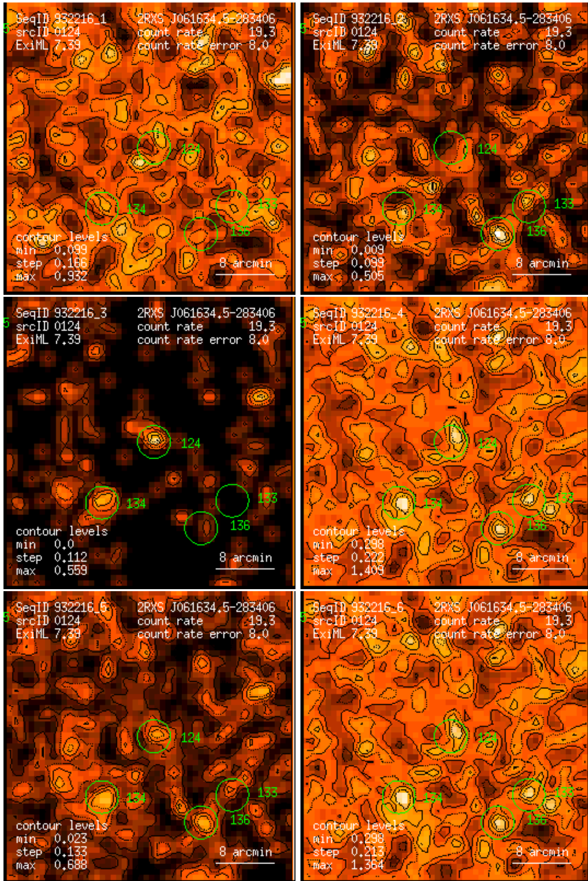
Figure 124: RASS 932216: detection 0124: band rate images, Gaussian filter: (1) PSPC channels 11 – 41, (2) 52 – 90, (3) 91 – 201, (4) 11 – 235, (5) 52 – 201, (6) 11 – 201. Broad band rates in counts/ks. Band rate contour levels in counts/ks/arcmin 2 .
