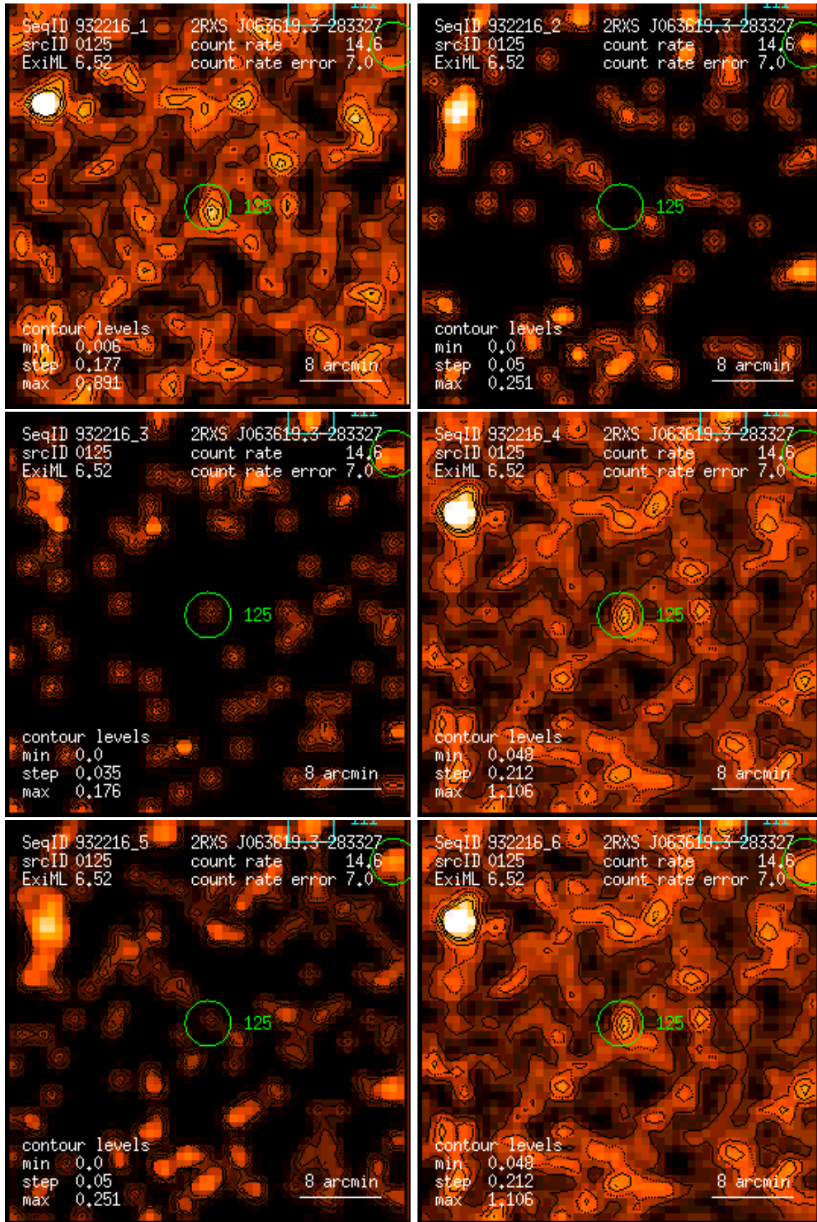
Figure 125: RASS 932216: detection 0125: band rate images, Gaussian filter: (1) PSPC channels 11 – 41, (2) 52 – 90, (3) 91 – 201, (4) 11 – 235, (5) 52 – 201, (6) 11 – 201. Broad band rates in counts/ks. Band rate contour levels in counts/ks/arcmin 2 .
