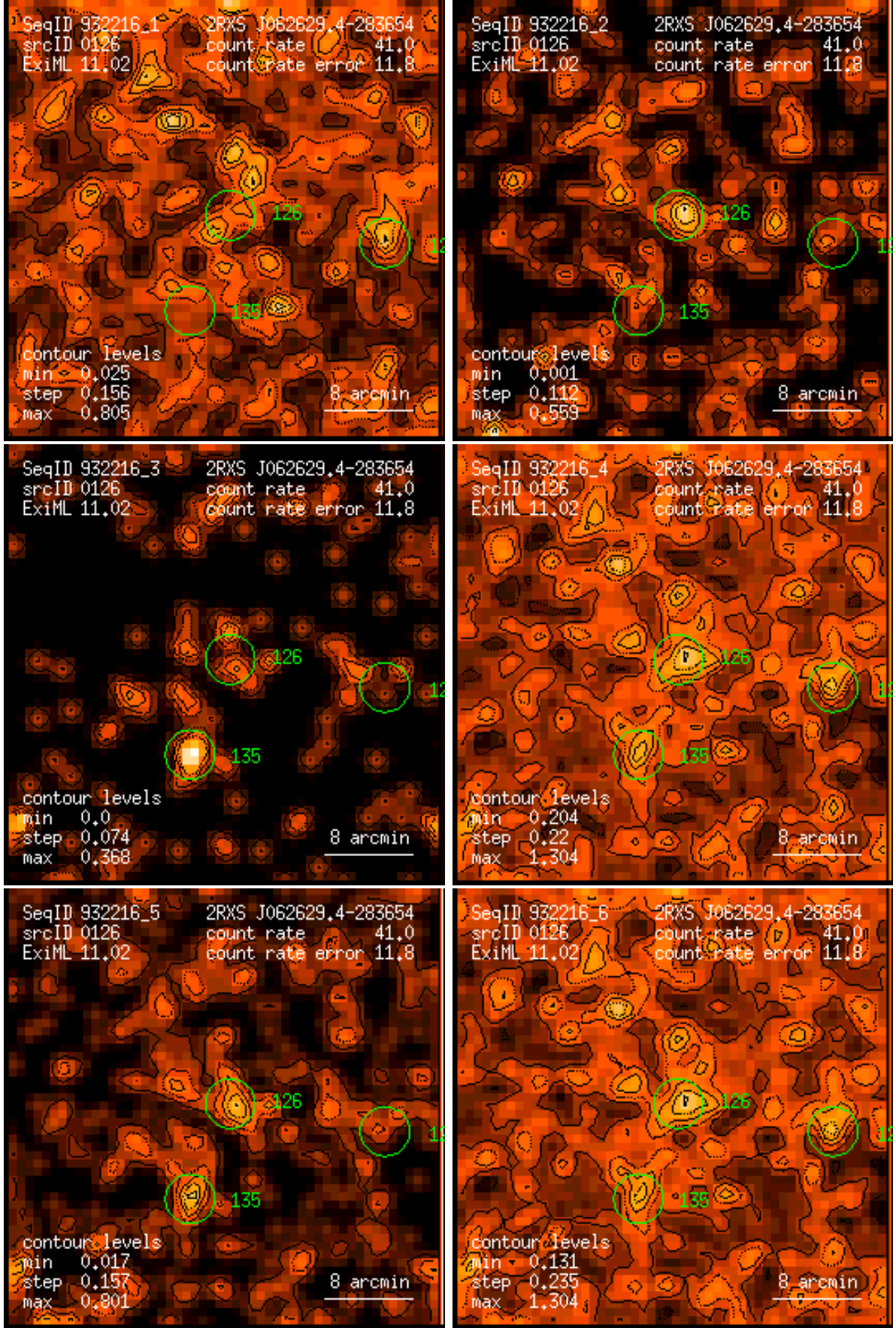
Figure 126: RASS 932216: detection 0126: band rate images, Gaussian filter: (1) PSPC channels 11 – 41, (2) 52 – 90, (3) 91 – 201, (4) 11 – 235, (5) 52 – 201, (6) 11 – 201. Broad band rates in counts/ks. Band rate contour levels in counts/ks/arcmin 2 .
