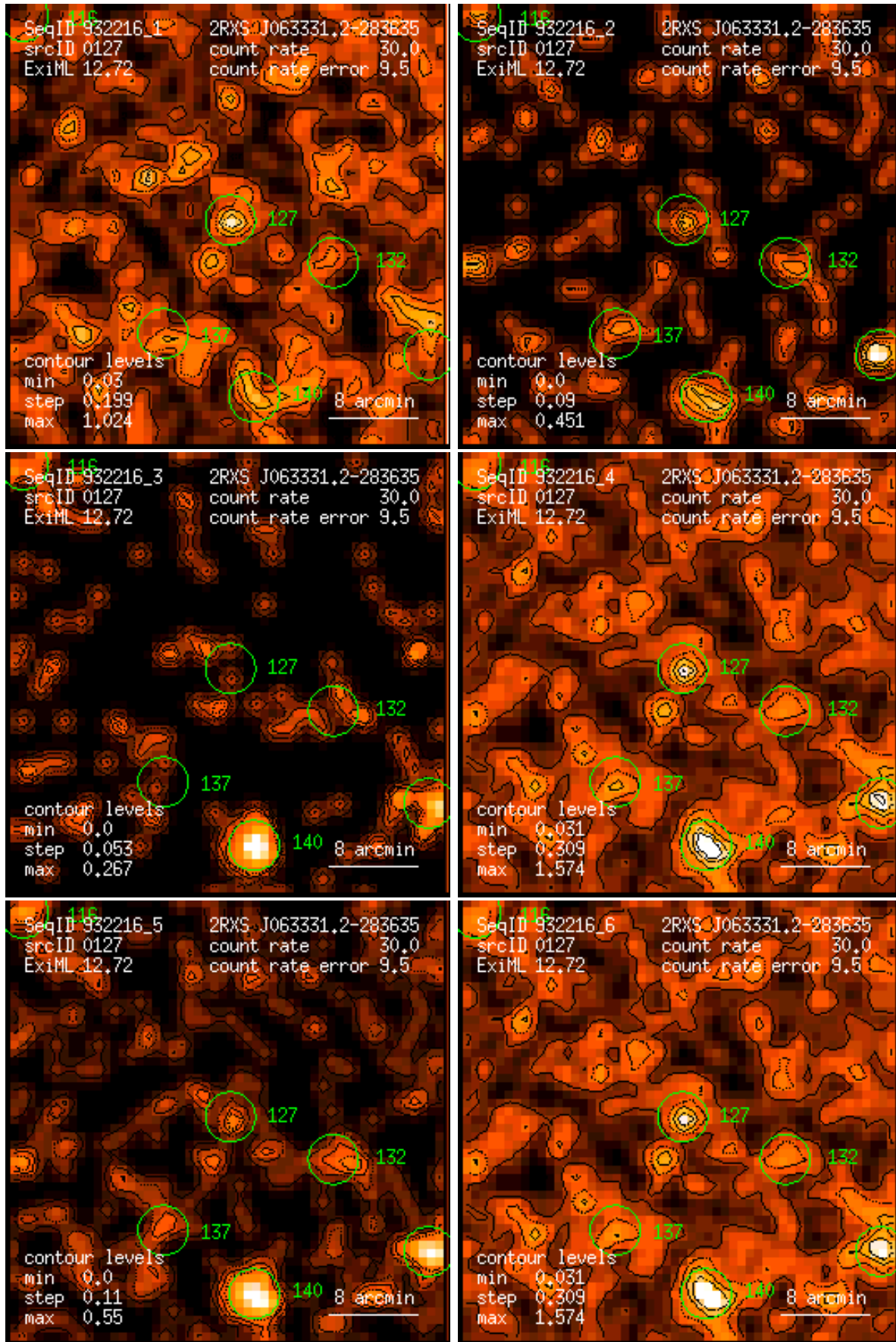
Figure 127: RASS 932216: detection 0127: band rate images, Gaussian filter: (1) PSPC channels 11 – 41, (2) 52 – 90, (3) 91 – 201, (4) 11 – 235, (5) 52 – 201, (6) 11 – 201. Broad band rates in counts/ks. Band rate contour levels in counts/ks/arcmin 2 .
