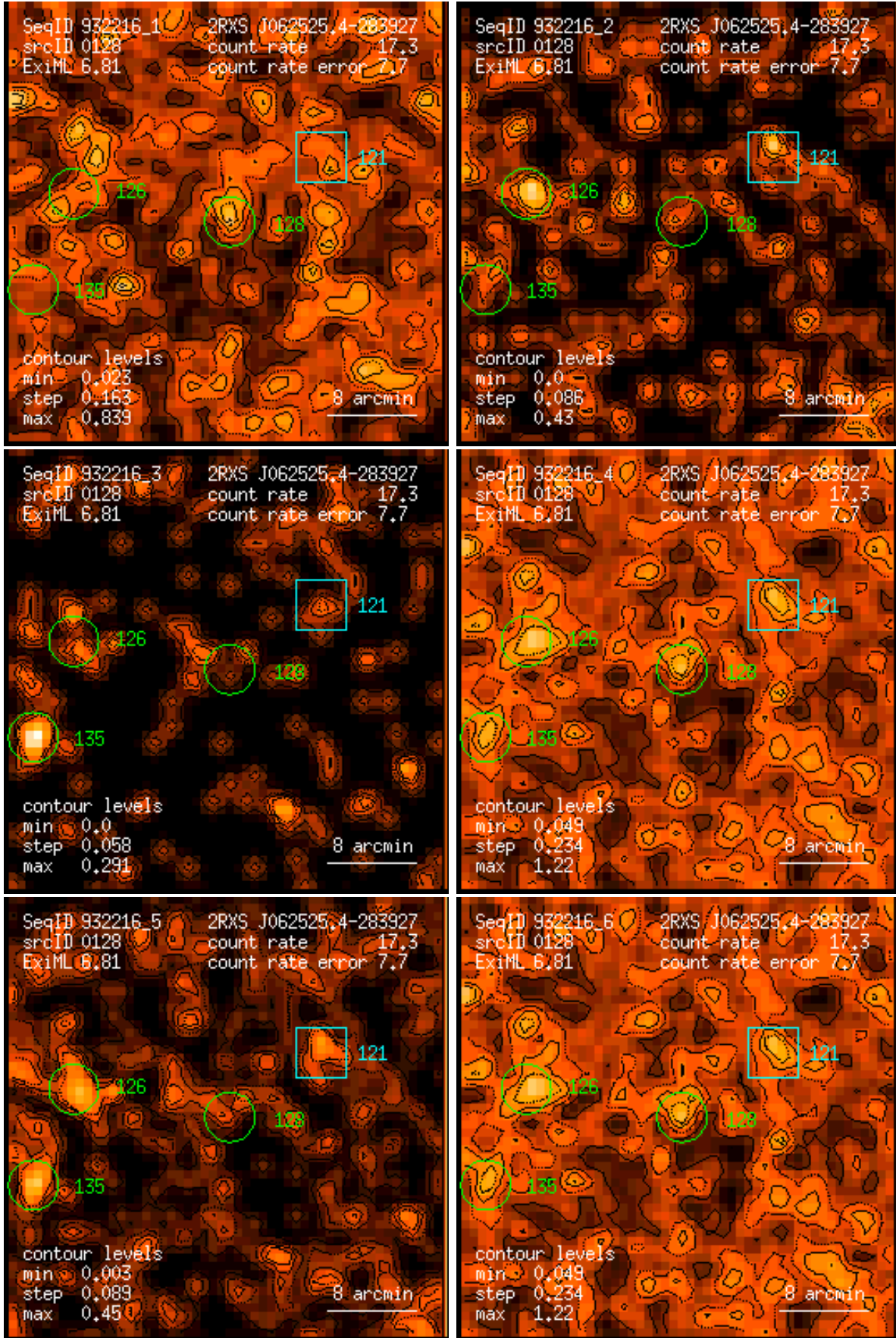
Figure 128: RASS 932216: detection 0128: band rate images, Gaussian filter: (1) PSPC channels 11 – 41, (2) 52 – 90, (3) 91 – 201, (4) 11 – 235, (5) 52 – 201, (6) 11 – 201. Broad band rates in counts/ks. Band rate contour levels in counts/ks/arcmin 2 .
