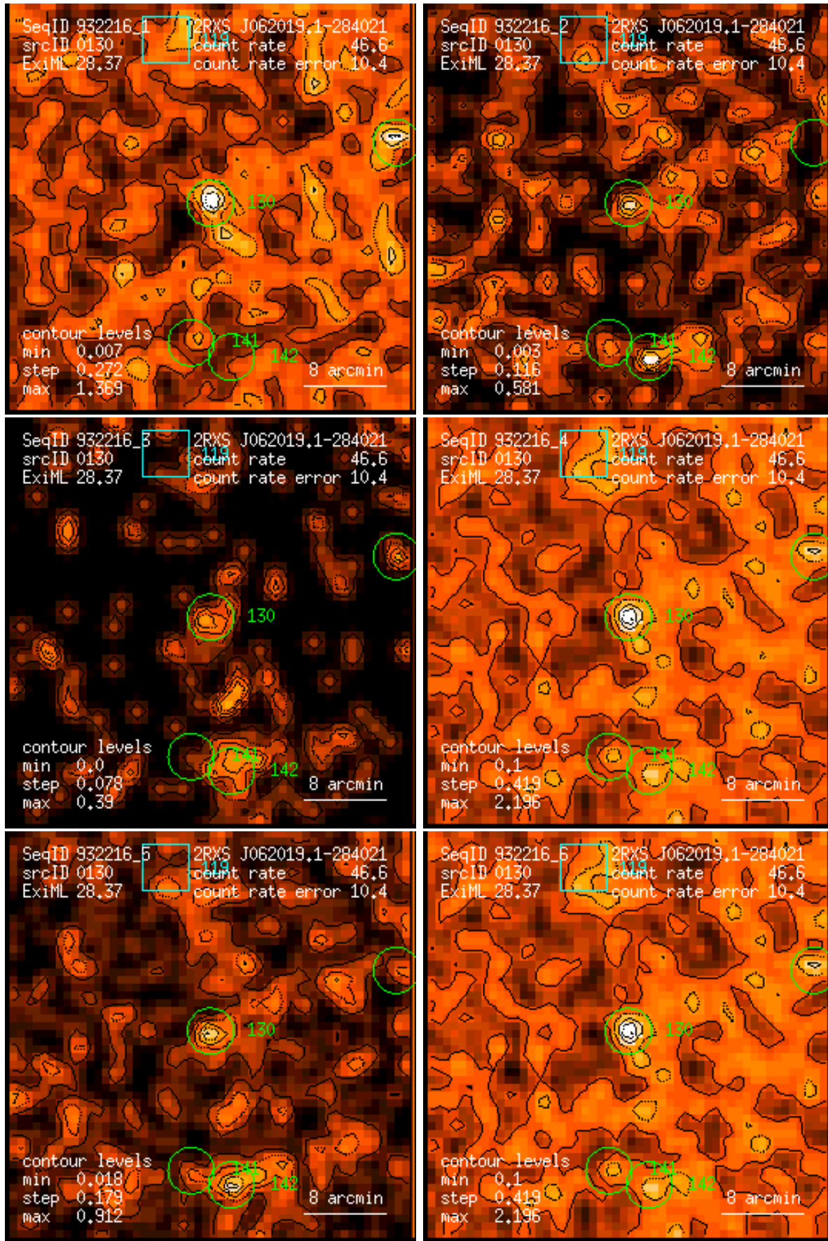
Figure 130: RASS 932216: detection 0130: band rate images, Gaussian filter: (1) PSPC channels 11 – 41, (2) 52 – 90, (3) 91 – 201, (4) 11 – 235, (5) 52 – 201, (6) 11 – 201. Broad band rates in counts/ks. Band rate contour levels in counts/ks/arcmin 2 .
