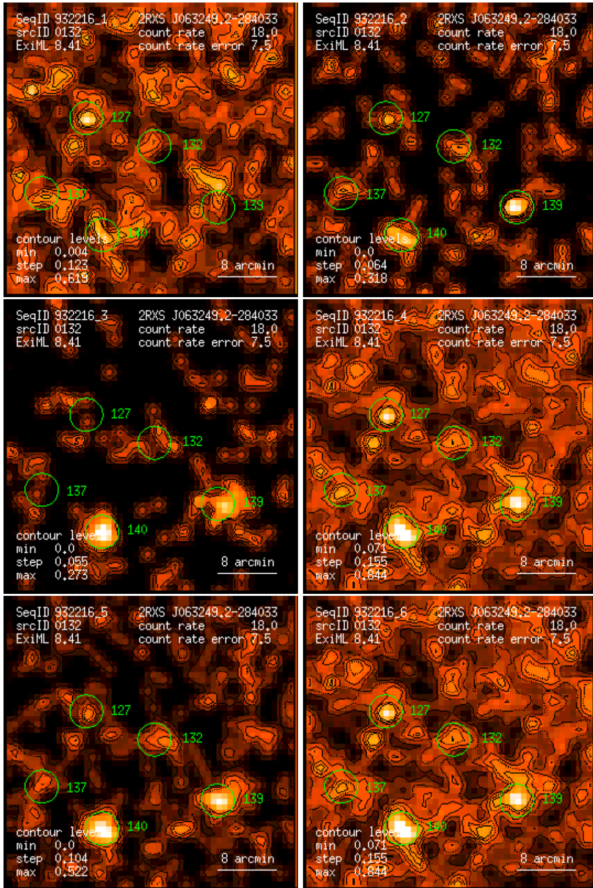
Figure 132: RASS 932216: detection 0132: band rate images, Gaussian filter: (1) PSPC channels 11 – 41, (2) 52 – 90, (3) 91 – 201, (4) 11 – 235, (5) 52 – 201, (6) 11 – 201. Broad band rates in counts/ks. Band rate contour levels in counts/ks/arcmin 2 .
