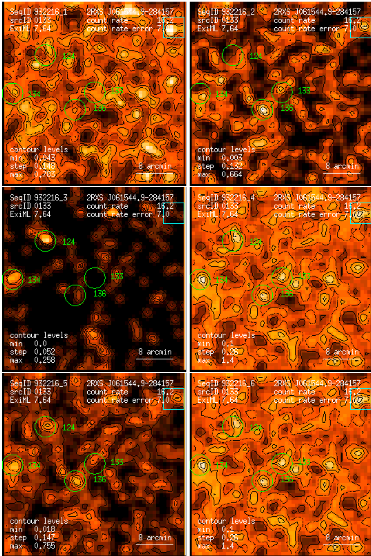
Figure 133: RASS 932216: detection 0133: band rate images, Gaussian filter: (1) PSPC channels 11 – 41, (2) 52 – 90, (3) 91 – 201, (4) 11 – 235, (5) 52 – 201, (6) 11 – 201. Broad band rates in counts/ks. Band rate contour levels in counts/ks/arcmin 2 .
