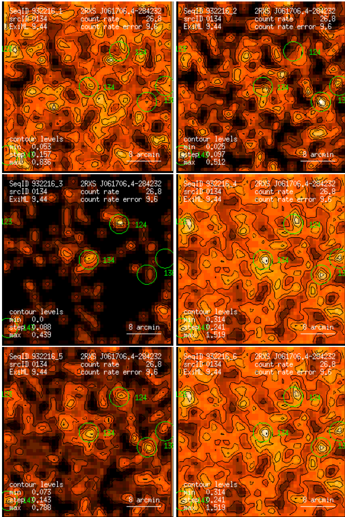
Figure 134: RASS 932216: detection 0134: band rate images, Gaussian filter: (1) PSPC channels 11 – 41, (2) 52 – 90, (3) 91 – 201, (4) 11 – 235, (5) 52 – 201, (6) 11 – 201. Broad band rates in counts/ks. Band rate contour levels in counts/ks/arcmin 2 .
