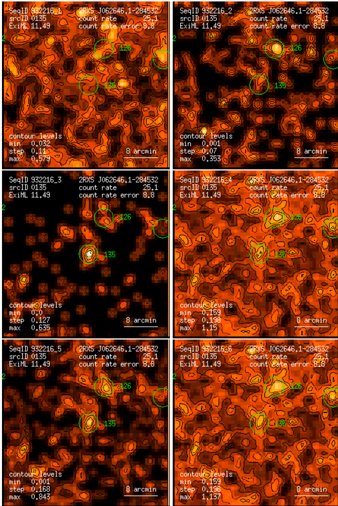
Figure 135: RASS 932216: detection 0135: band rate images, Gaussian filter: (1) PSPC channels 11 – 41, (2) 52 – 90, (3) 91 – 201, (4) 11 – 235, (5) 52 – 201, (6) 11 – 201. Broad band rates in counts/ks. Band rate contour levels in counts/ks/arcmin 2 .
