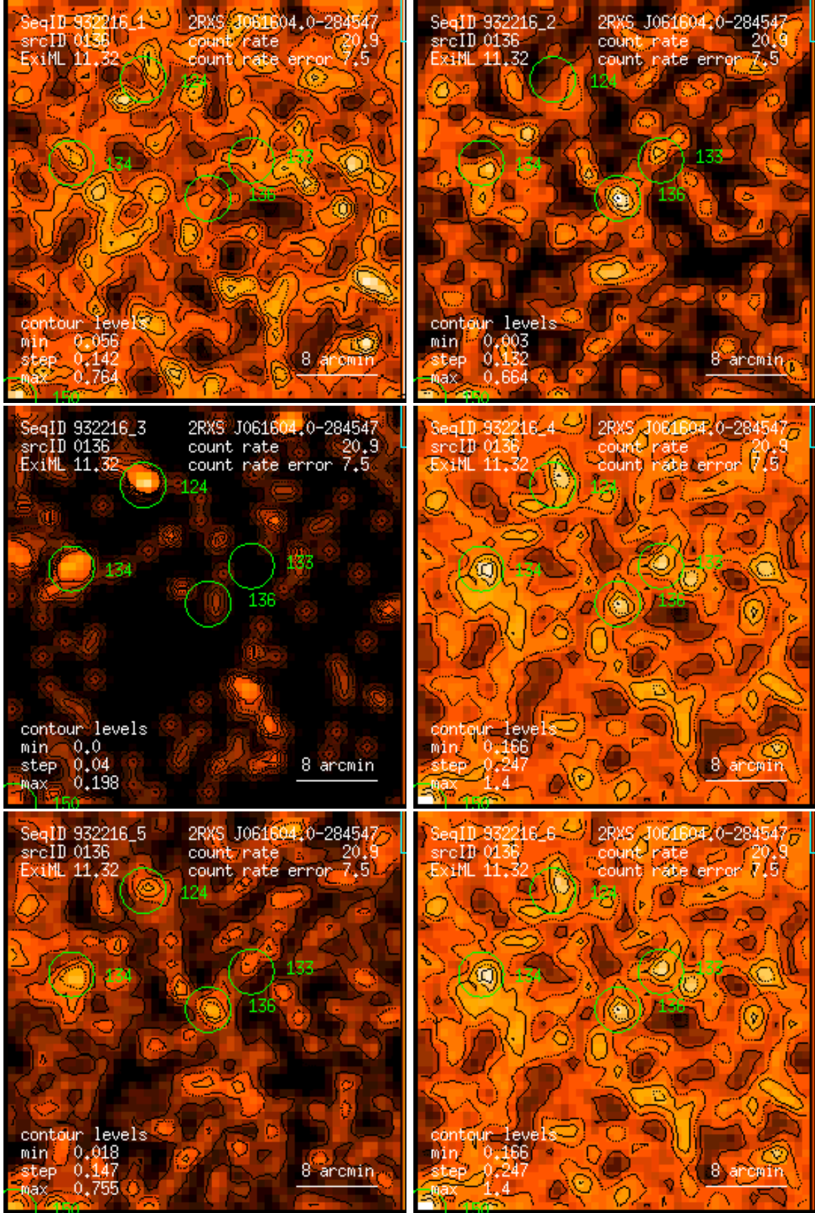
Figure 136: RASS 932216: detection 0136: band rate images, Gaussian filter: (1) PSPC channels 11 – 41, (2) 52 – 90, (3) 91 – 201, (4) 11 – 235, (5) 52 – 201, (6) 11 – 201. Broad band rates in counts/ks. Band rate contour levels in counts/ks/arcmin 2 .
