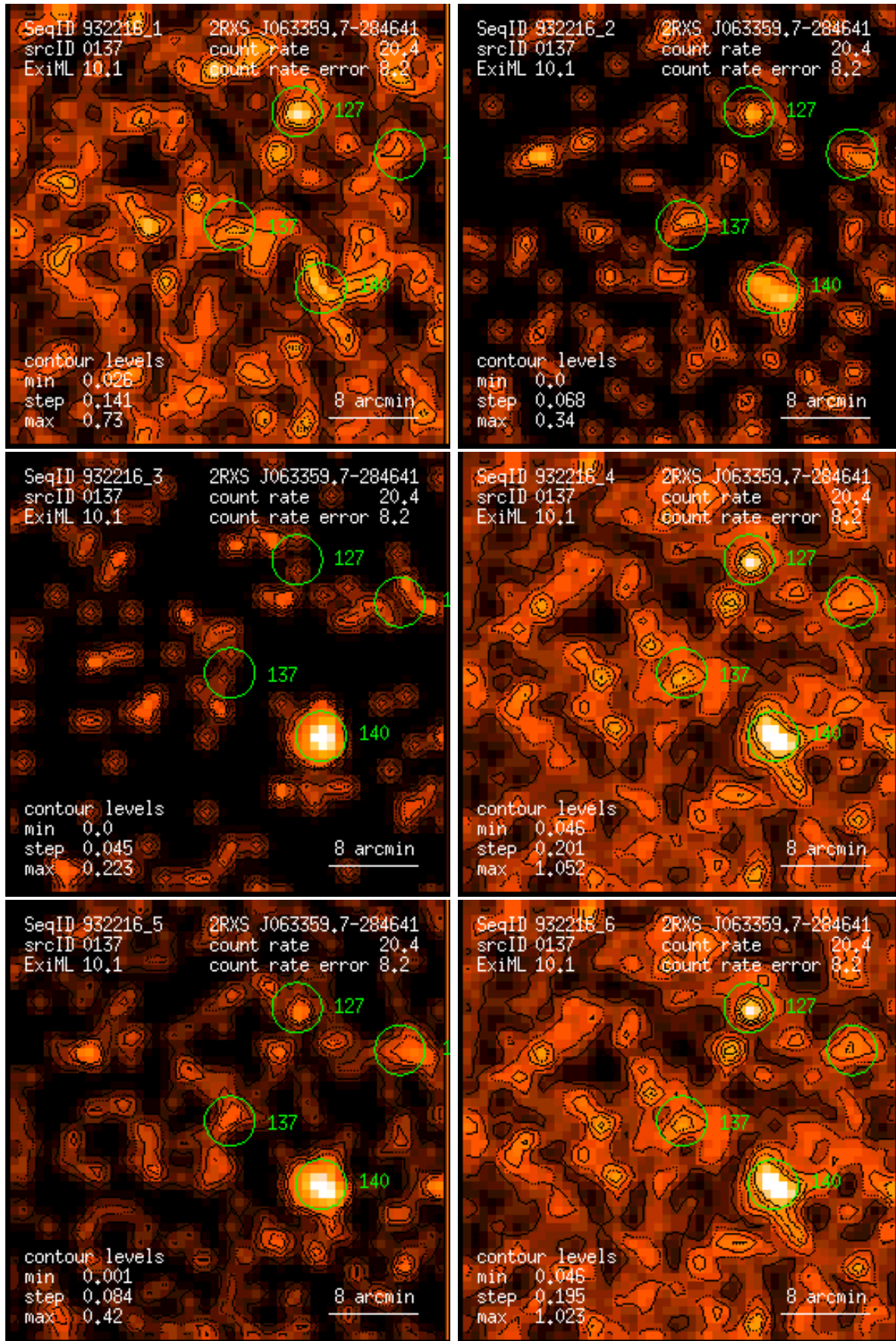
Figure 137: RASS 932216: detection 0137: band rate images, Gaussian filter: (1) PSPC channels 11 – 41, (2) 52 – 90, (3) 91 – 201, (4) 11 – 235, (5) 52 – 201, (6) 11 – 201. Broad band rates in counts/ks. Band rate contour levels in counts/ks/arcmin 2 .
