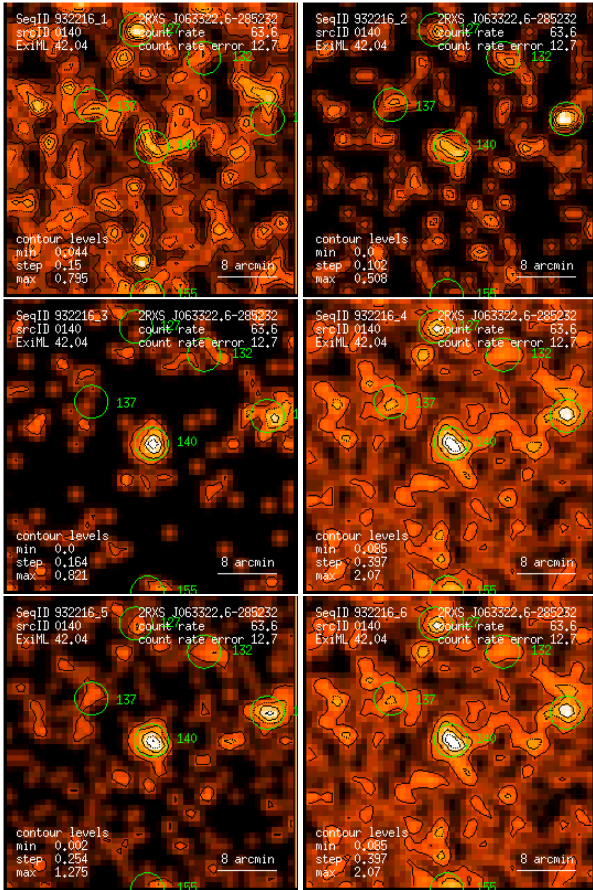
Figure 140: RASS 932216: detection 0140: band rate images, Gaussian filter: (1) PSPC channels 11 – 41, (2) 52 – 90, (3) 91 – 201, (4) 11 – 235, (5) 52 – 201, (6) 11 – 201. Broad band rates in counts/ks. Band rate contour levels in counts/ks/arcmin 2 .
