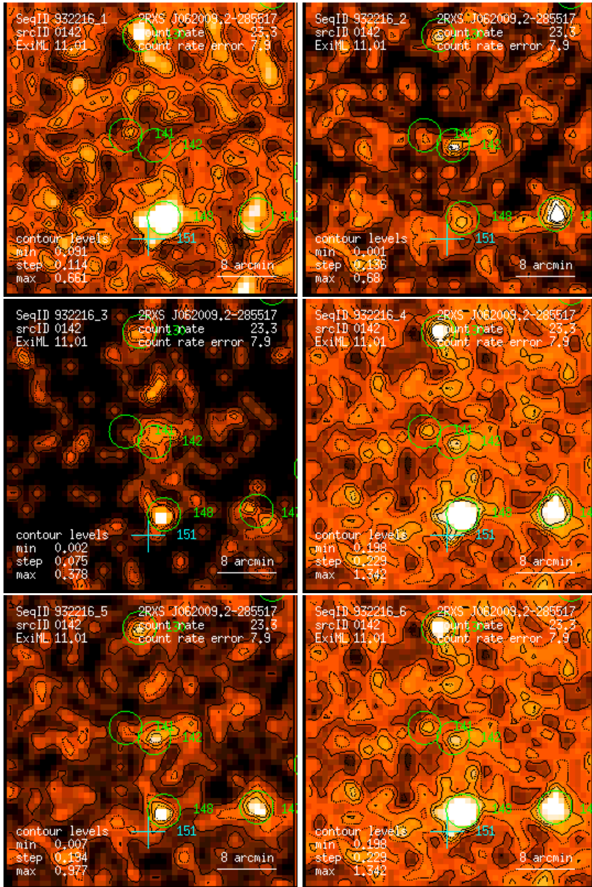
Figure 142: RASS 932216: detection 0142: band rate images, Gaussian filter: (1) PSPC channels 11 – 41, (2) 52 – 90, (3) 91 – 201, (4) 11 – 235, (5) 52 – 201, (6) 11 – 201. Broad band rates in counts/ks. Band rate contour levels in counts/ks/arcmin 2 .
