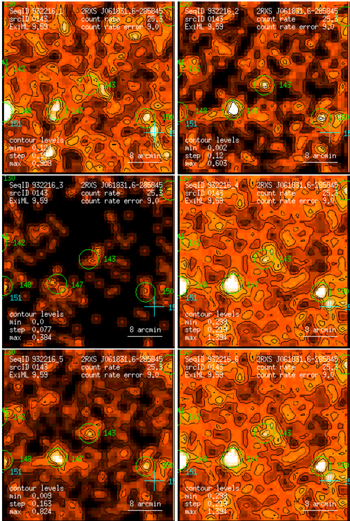
Figure 143: RASS 932216: detection 0143: band rate images, Gaussian filter: (1) PSPC channels 11 – 41, (2) 52 – 90, (3) 91 – 201, (4) 11 – 235, (5) 52 – 201, (6) 11 – 201. Broad band rates in counts/ks. Band rate contour levels in counts/ks/arcmin 2 .
