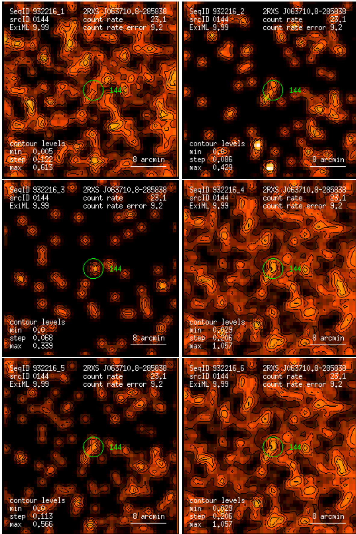
Figure 144: RASS 932216: detection 0144: band rate images, Gaussian filter: (1) PSPC channels 11 – 41, (2) 52 – 90, (3) 91 – 201, (4) 11 – 235, (5) 52 – 201, (6) 11 – 201. Broad band rates in counts/ks. Band rate contour levels in counts/ks/arcmin 2 .
