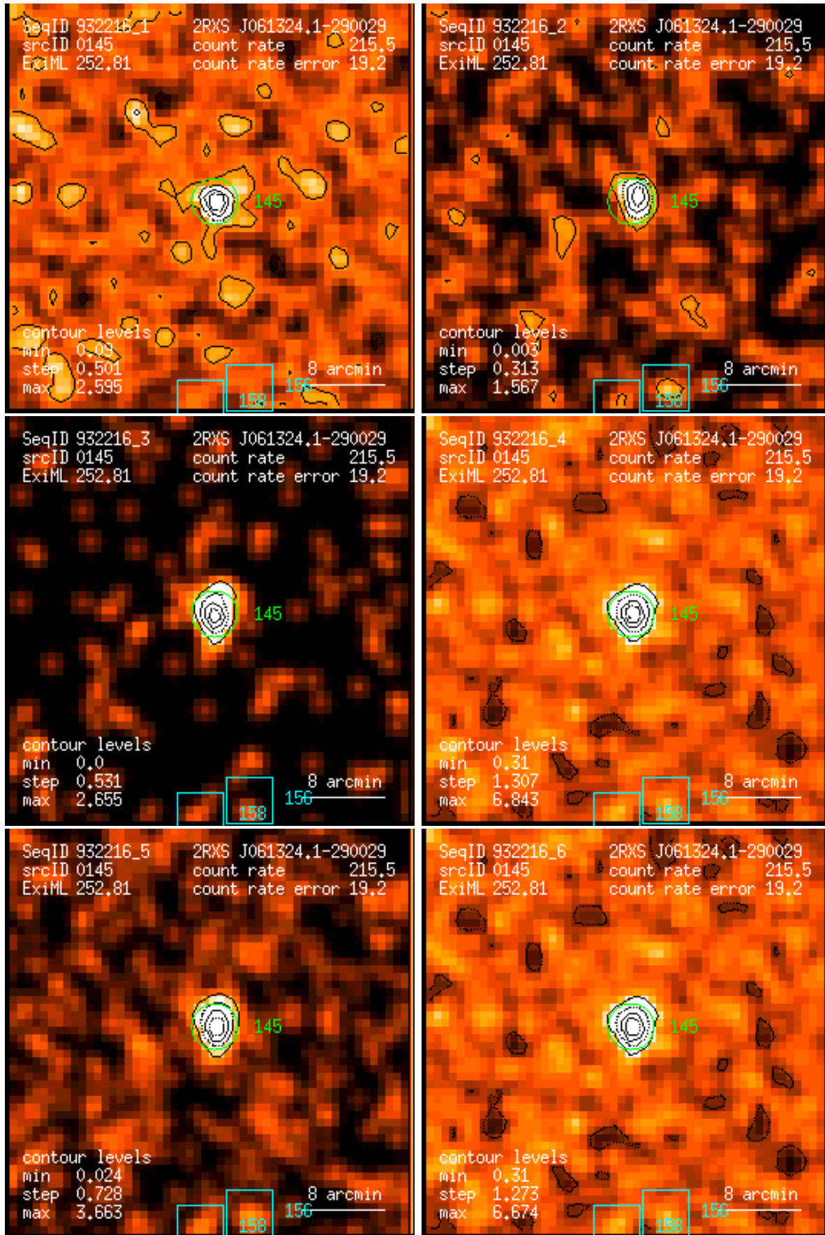
Figure 145: RASS 932216: detection 0145: band rate images, Gaussian filter: (1) PSPC channels 11 – 41, (2) 52 – 90, (3) 91 – 201, (4) 11 – 235, (5) 52 – 201, (6) 11 – 201. Broad band rates in counts/ks. Band rate contour levels in counts/ks/arcmin 2 .
