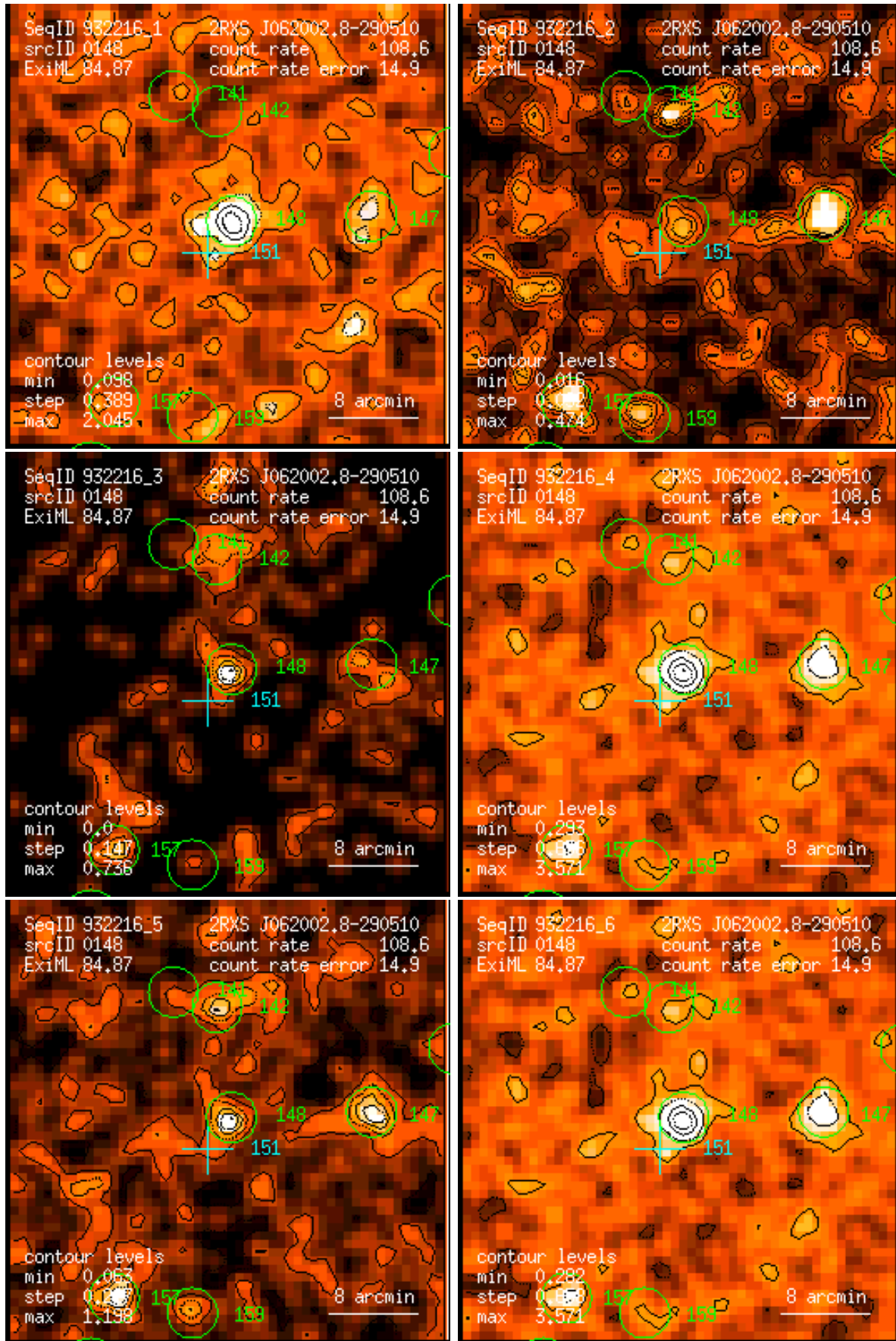
Figure 148: RASS 932216: detection 0148: band rate images, Gaussian filter: (1) PSPC channels 11 – 41, (2) 52 – 90, (3) 91 – 201, (4) 11 – 235, (5) 52 – 201, (6) 11 – 201. Broad band rates in counts/ks. Band rate contour levels in counts/ks/arcmin 2 .
