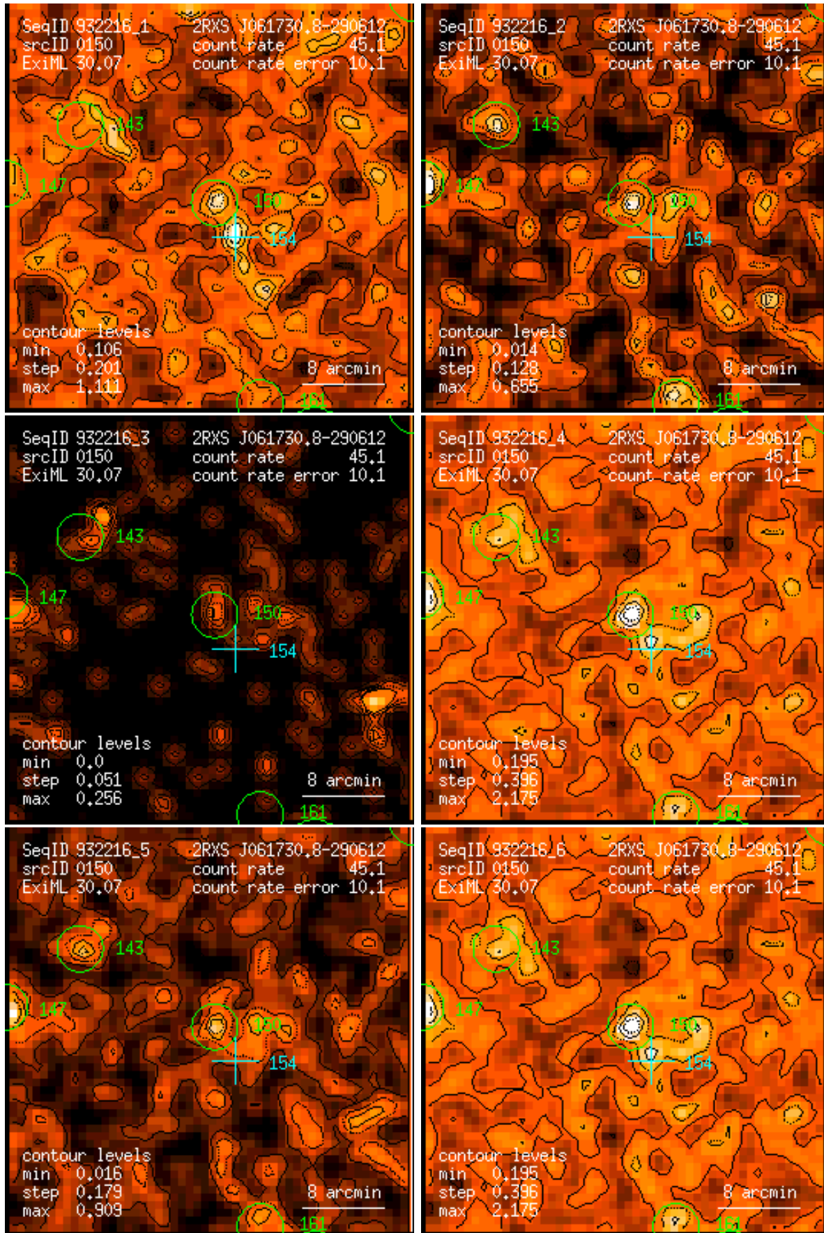
Figure 150: RASS 932216: detection 0150: band rate images, Gaussian filter: (1) PSPC channels 11 – 41, (2) 52 – 90, (3) 91 – 201, (4) 11 – 235, (5) 52 – 201, (6) 11 – 201. Broad band rates in counts/ks. Band rate contour levels in counts/ks/arcmin 2 .
