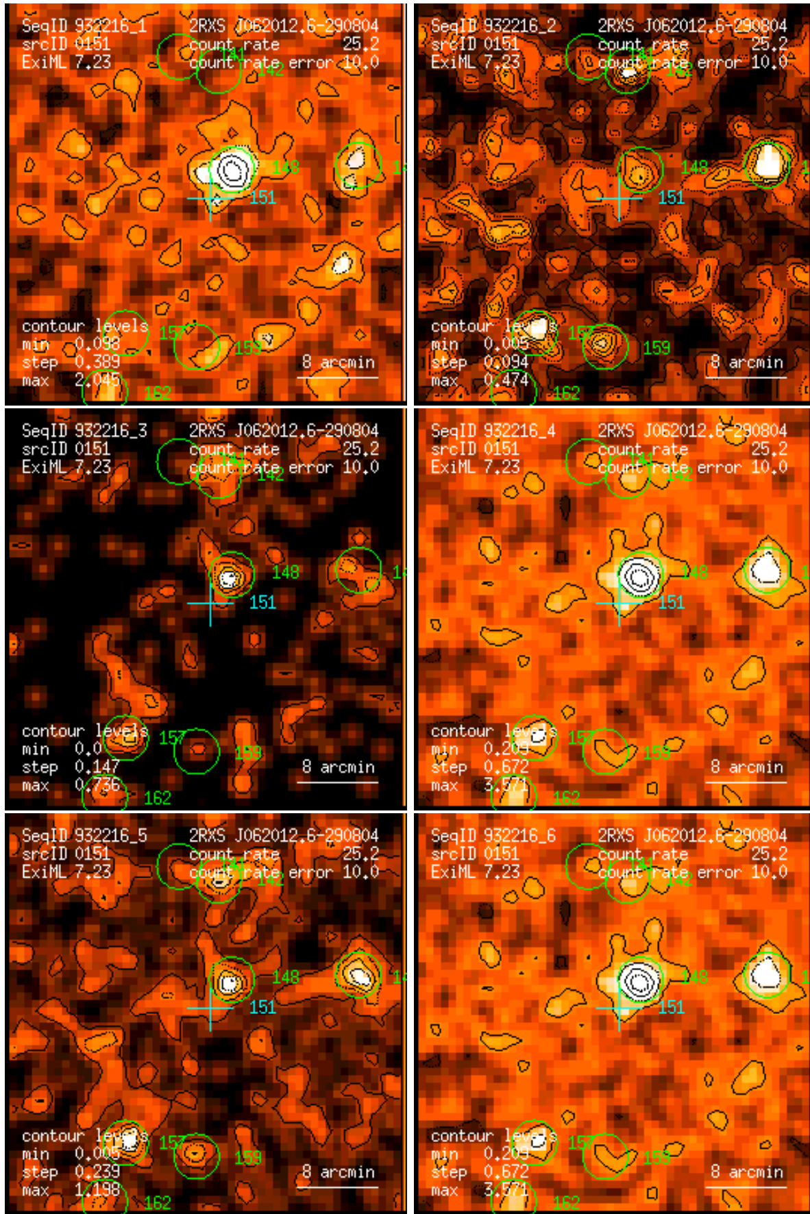
Figure 151: RASS 932216: detection 0151: band rate images, Gaussian filter: (1) PSPC channels 11 – 41, (2) 52 – 90, (3) 91 – 201, (4) 11 – 235, (5) 52 – 201, (6) 11 – 201. Broad band rates in counts/ks. Band rate contour levels in counts/ks/arcmin 2 .
