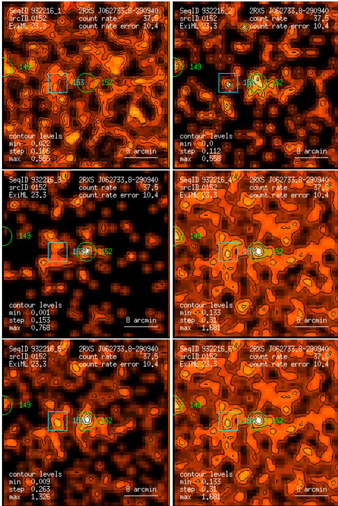
Figure 152: RASS 932216: detection 0152: band rate images, Gaussian filter: (1) PSPC channels 11 – 41, (2) 52 – 90, (3) 91 – 201, (4) 11 – 235, (5) 52 – 201, (6) 11 – 201. Broad band rates in counts/ks. Band rate contour levels in counts/ks/arcmin 2 .
