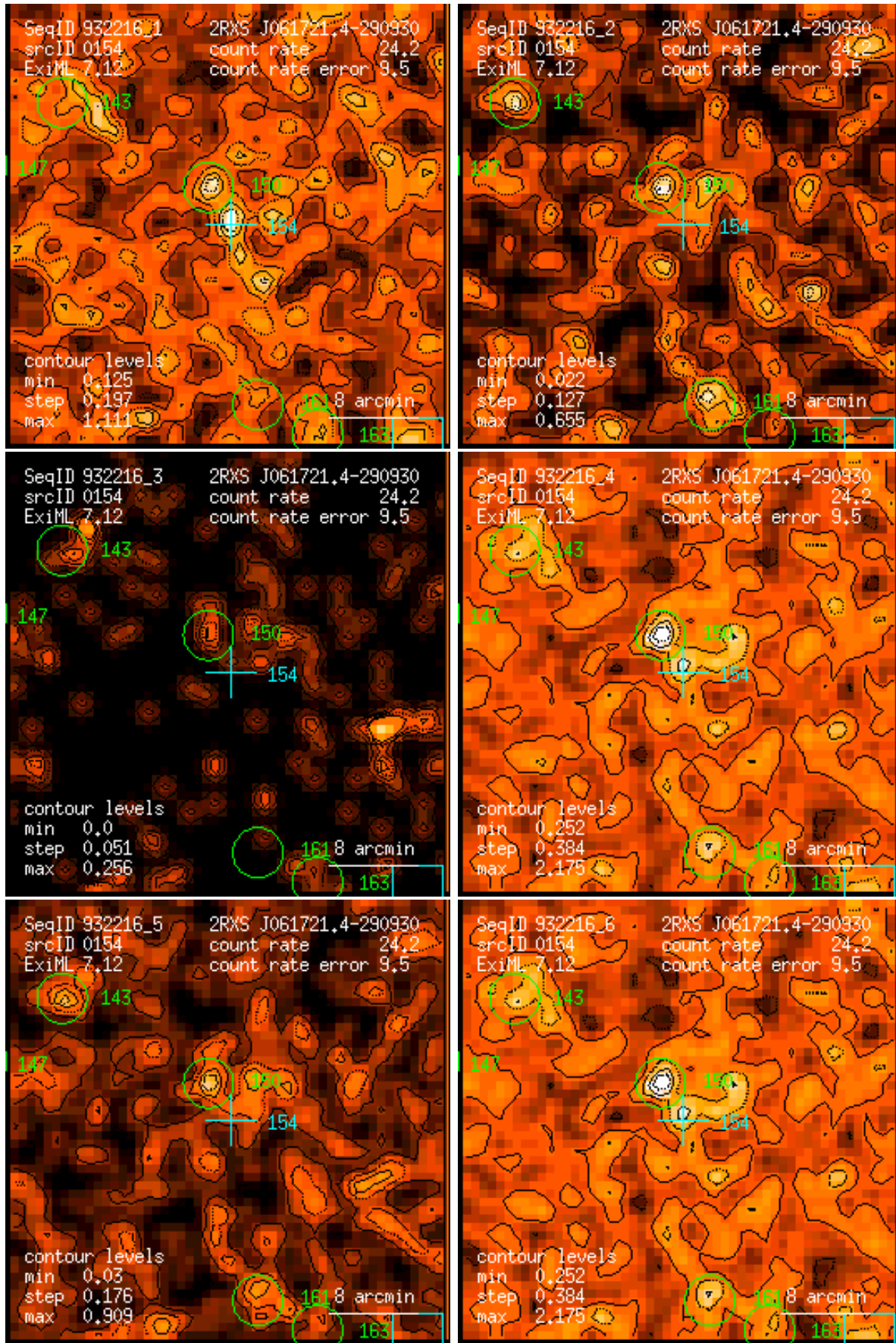
Figure 154: RASS 932216: detection 0154: band rate images, Gaussian filter: (1) PSPC channels 11 – 41, (2) 52 – 90, (3) 91 – 201, (4) 11 – 235, (5) 52 – 201, (6) 11 – 201. Broad band rates in counts/ks. Band rate contour levels in counts/ks/arcmin 2 .
