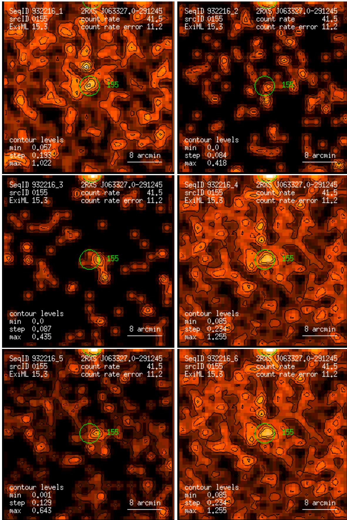
Figure 155: RASS 932216: detection 0155: band rate images, Gaussian filter: (1) PSPC channels 11 – 41, (2) 52 – 90, (3) 91 – 201, (4) 11 – 235, (5) 52 – 201, (6) 11 – 201. Broad band rates in counts/ks. Band rate contour levels in counts/ks/arcmin 2 .
