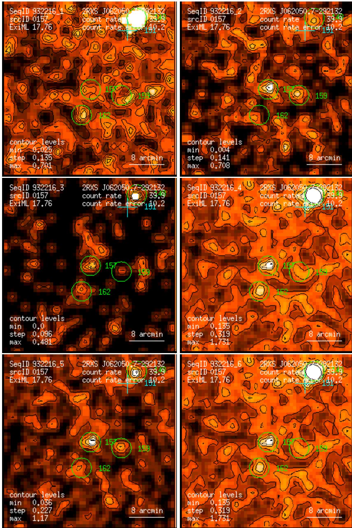
Figure 157: RASS 932216: detection 0157: band rate images, Gaussian filter: (1) PSPC channels 11 – 41, (2) 52 – 90, (3) 91 – 201, (4) 11 – 235, (5) 52 – 201, (6) 11 – 201. Broad band rates in counts/ks. Band rate contour levels in counts/ks/arcmin 2 .
