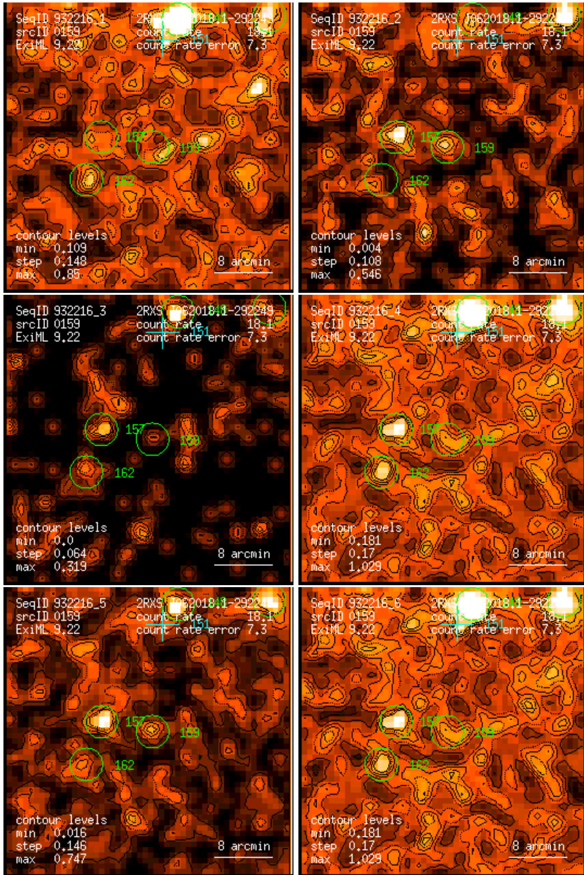
Figure 159: RASS 932216: detection 0159: band rate images, Gaussian filter: (1) PSPC channels 11 – 41, (2) 52 – 90, (3) 91 – 201, (4) 11 – 235, (5) 52 – 201, (6) 11 – 201. Broad band rates in counts/ks. Band rate contour levels in counts/ks/arcmin 2 .
