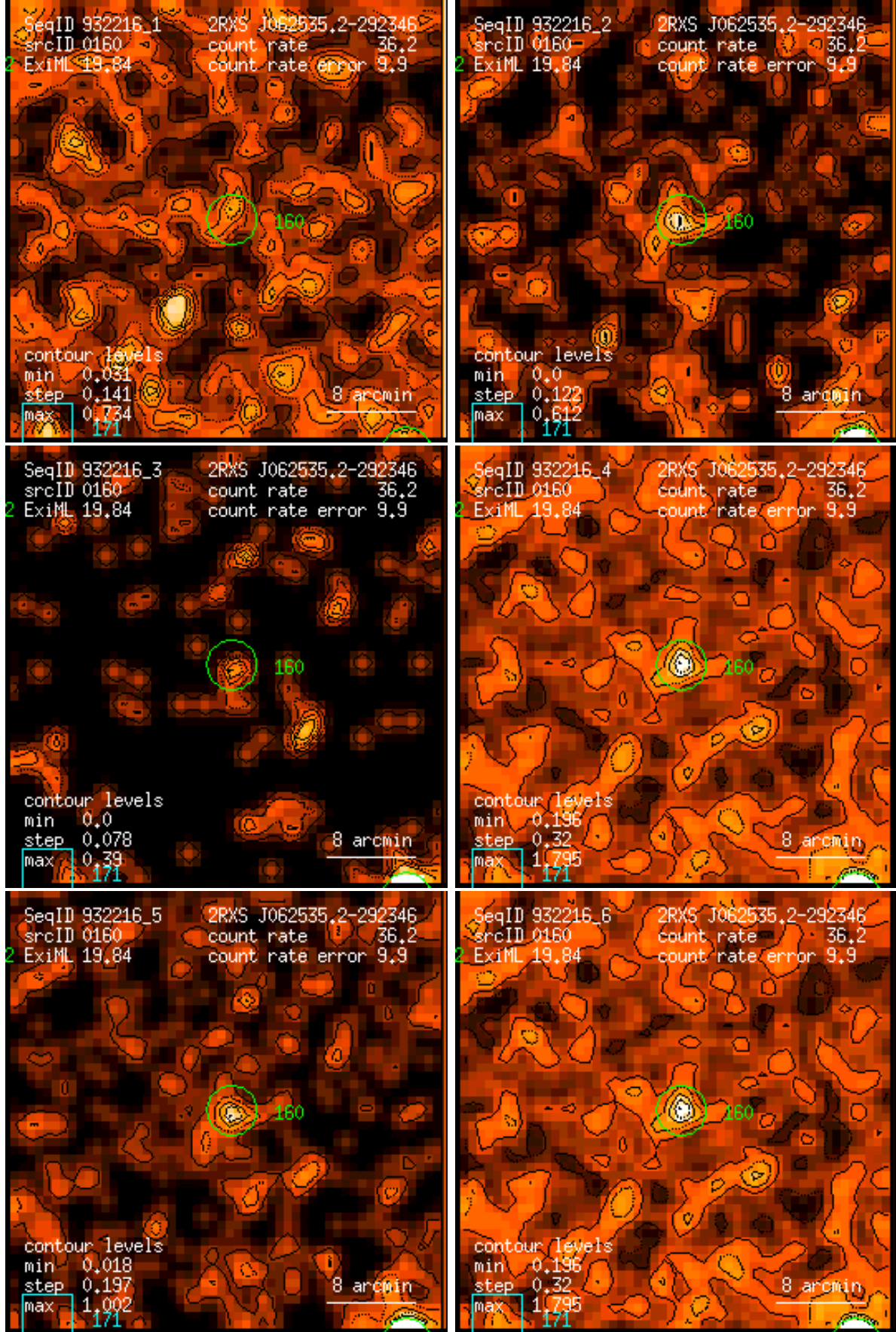
Figure 160: RASS 932216: detection 0160: band rate images, Gaussian filter: (1) PSPC channels 11 – 41, (2) 52 – 90, (3) 91 – 201, (4) 11 – 235, (5) 52 – 201, (6) 11 – 201. Broad band rates in counts/ks. Band rate contour levels in counts/ks/arcmin 2 .
