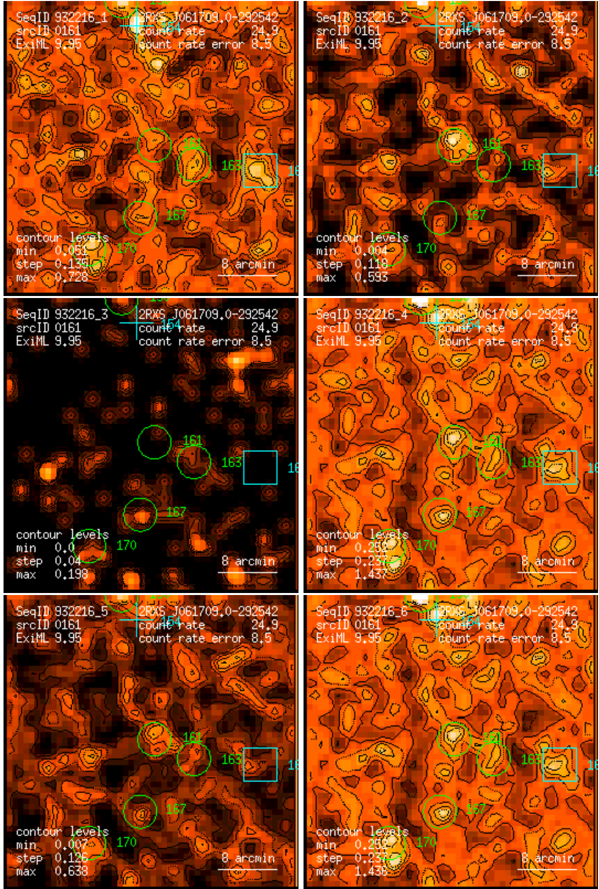
Figure 161: RASS 932216: detection 0161: band rate images, Gaussian filter: (1) PSPC channels 11 – 41, (2) 52 – 90, (3) 91 – 201, (4) 11 – 235, (5) 52 – 201, (6) 11 – 201. Broad band rates in counts/ks. Band rate contour levels in counts/ks/arcmin 2 .
