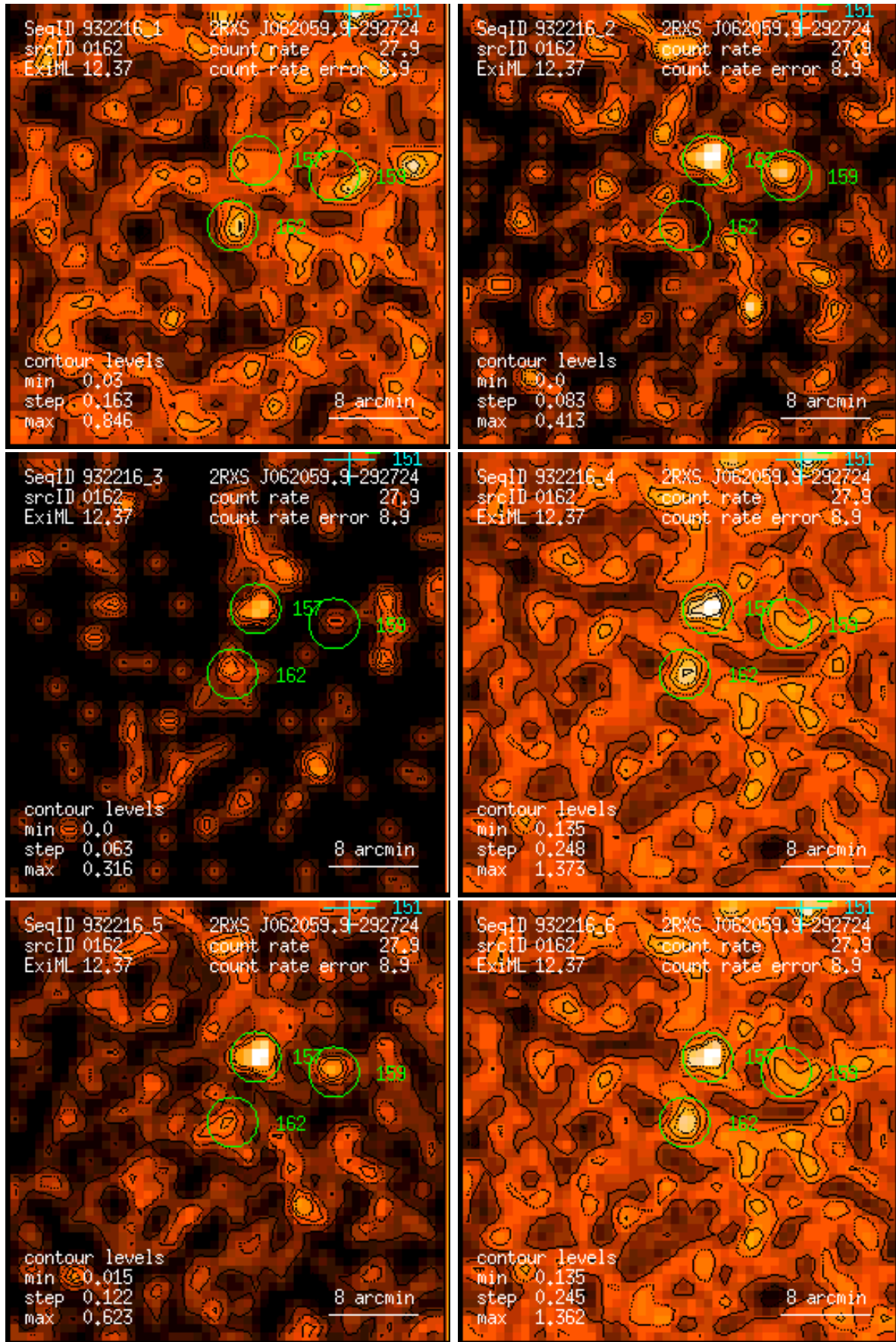
Figure 162: RASS 932216: detection 0162: band rate images, Gaussian filter: (1) PSPC channels 11 – 41, (2) 52 – 90, (3) 91 – 201, (4) 11 – 235, (5) 52 – 201, (6) 11 – 201. Broad band rates in counts/ks. Band rate contour levels in counts/ks/arcmin 2 .
