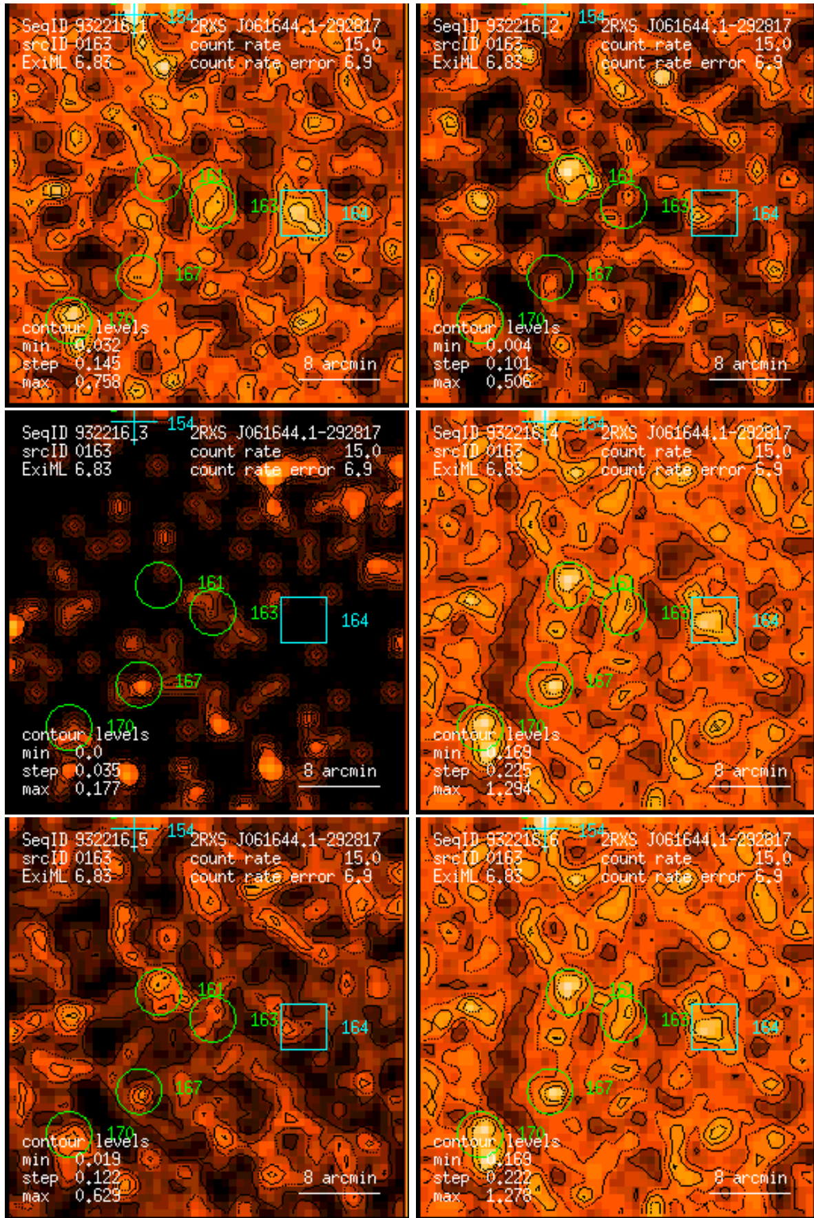
Figure 163: RASS 932216: detection 0163: band rate images, Gaussian filter: (1) PSPC channels 11 – 41, (2) 52 – 90, (3) 91 – 201, (4) 11 – 235, (5) 52 – 201, (6) 11 – 201. Broad band rates in counts/ks. Band rate contour levels in counts/ks/arcmin 2 .
