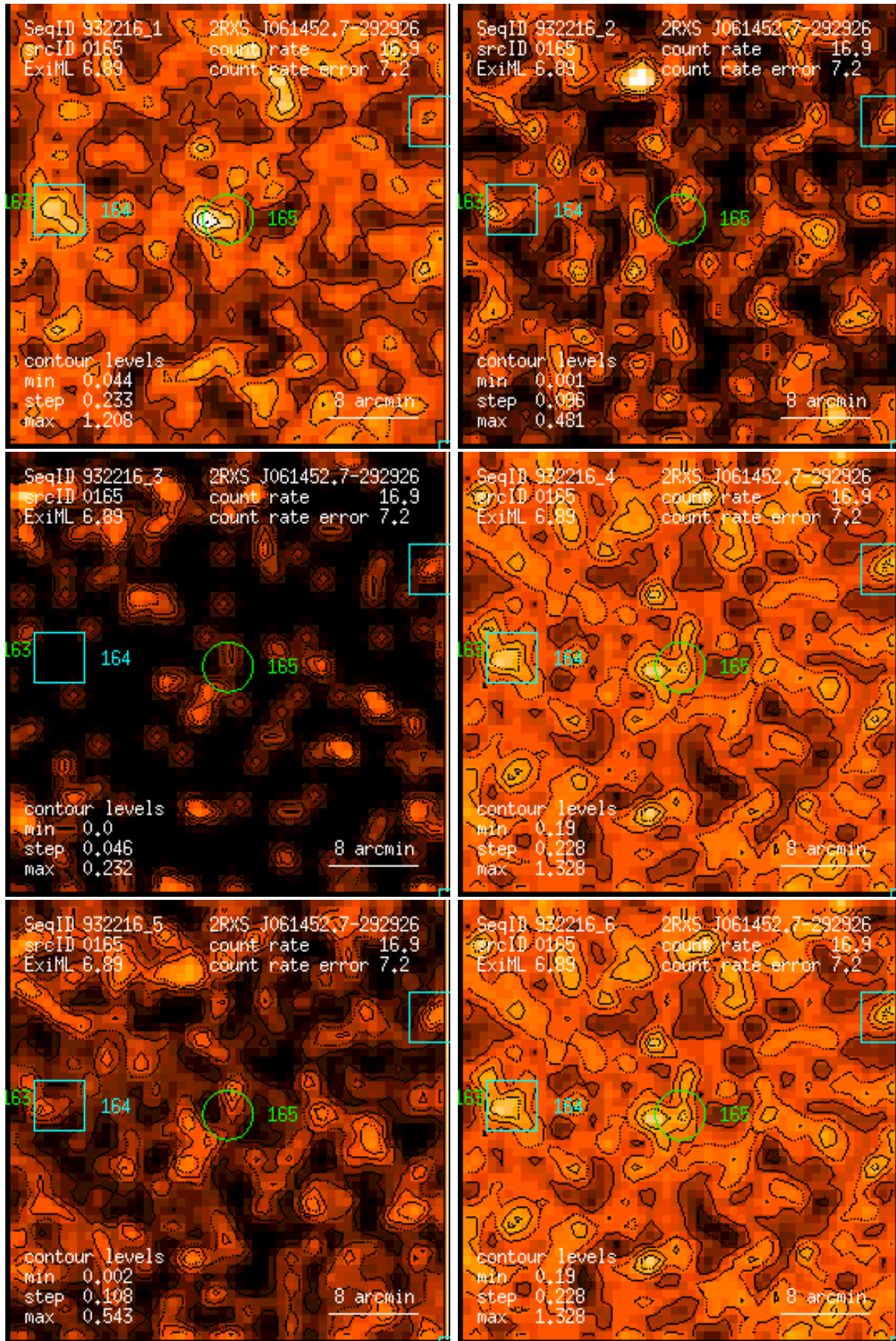
Figure 165: RASS 932216: detection 0165: band rate images, Gaussian filter: (1) PSPC channels 11 – 41, (2) 52 – 90, (3) 91 – 201, (4) 11 – 235, (5) 52 – 201, (6) 11 – 201. Broad band rates in counts/ks. Band rate contour levels in counts/ks/arcmin 2 .
