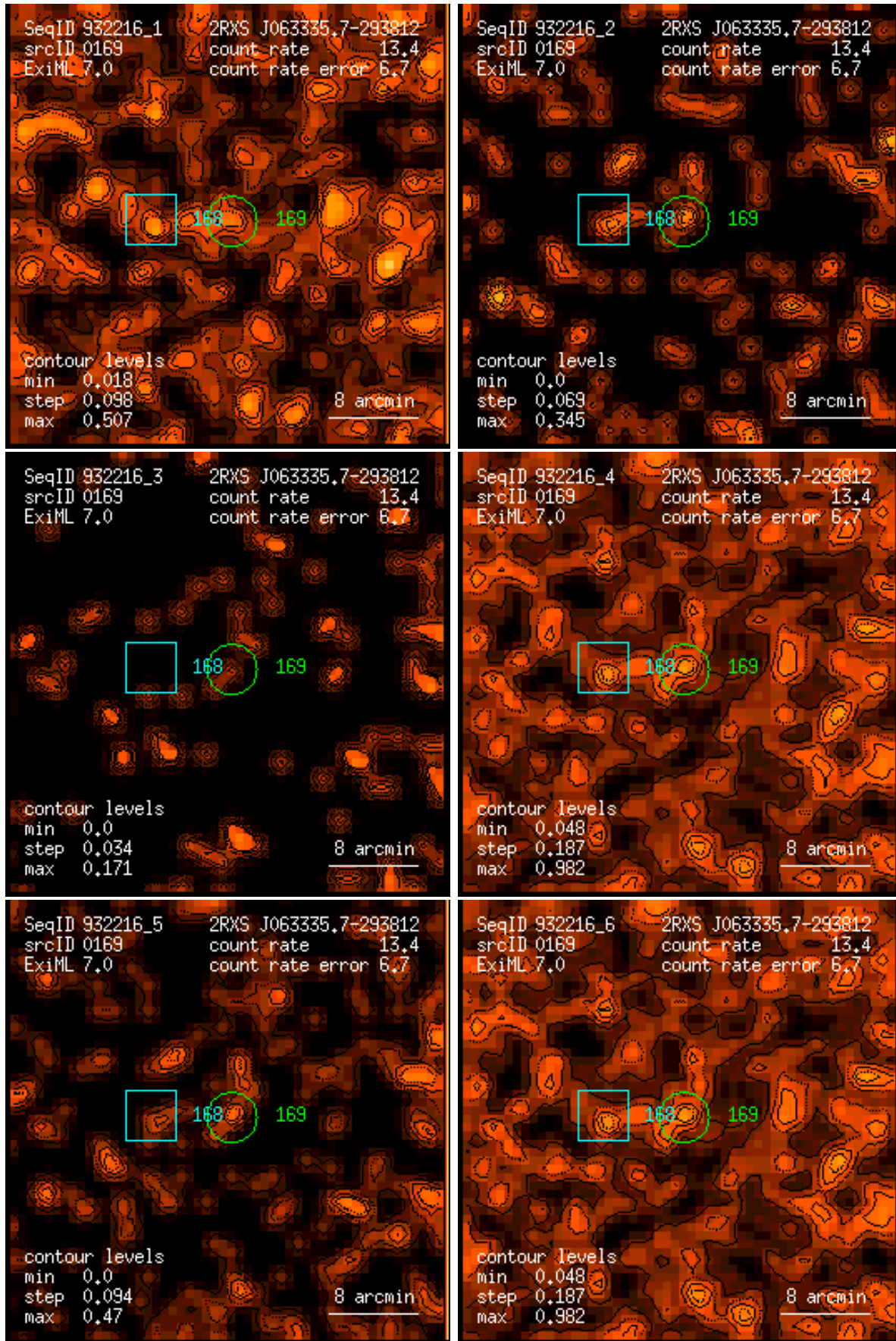
Figure 169: RASS 932216: detection 0169: band rate images, Gaussian filter: (1) PSPC channels 11 – 41, (2) 52 – 90, (3) 91 – 201, (4) 11 – 235, (5) 52 – 201, (6) 11 – 201. Broad band rates in counts/ks. Band rate contour levels in counts/ks/arcmin 2 .
