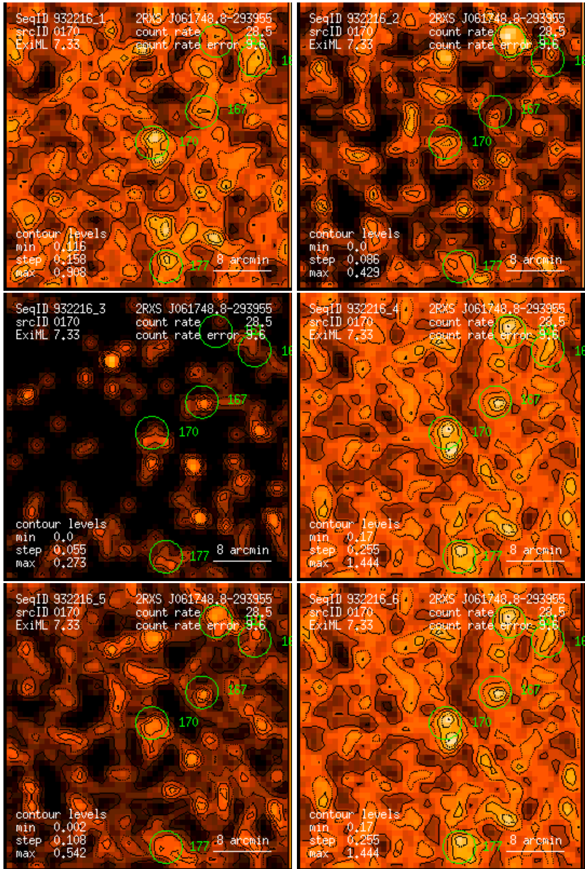
Figure 170: RASS 932216: detection 0170: band rate images, Gaussian filter: (1) PSPC channels 11 – 41, (2) 52 – 90, (3) 91 – 201, (4) 11 – 235, (5) 52 – 201, (6) 11 – 201. Broad band rates in counts/ks. Band rate contour levels in counts/ks/arcmin 2 .
