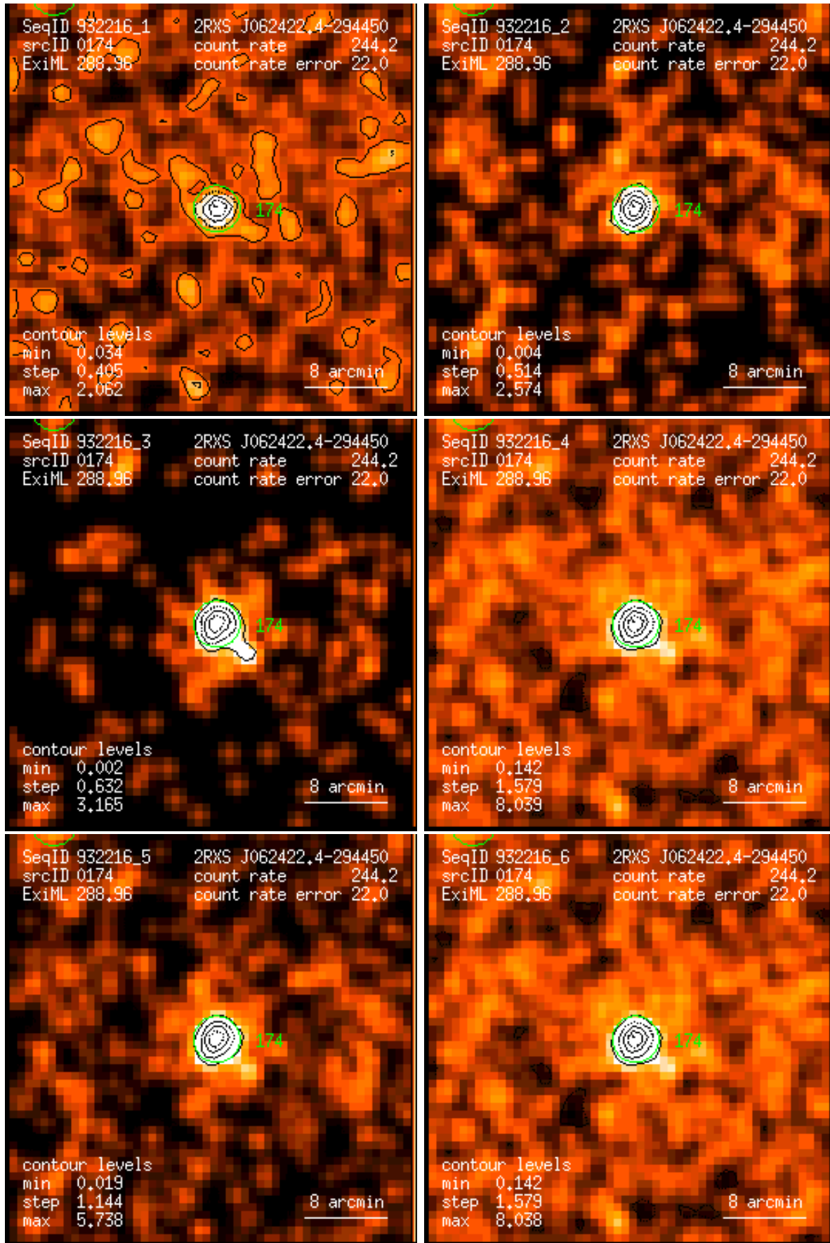
Figure 174: RASS 932216: detection 0174: band rate images, Gaussian filter: (1) PSPC channels 11 – 41, (2) 52 – 90, (3) 91 – 201, (4) 11 – 235, (5) 52 – 201, (6) 11 – 201. Broad band rates in counts/ks. Band rate contour levels in counts/ks/arcmin 2 .
