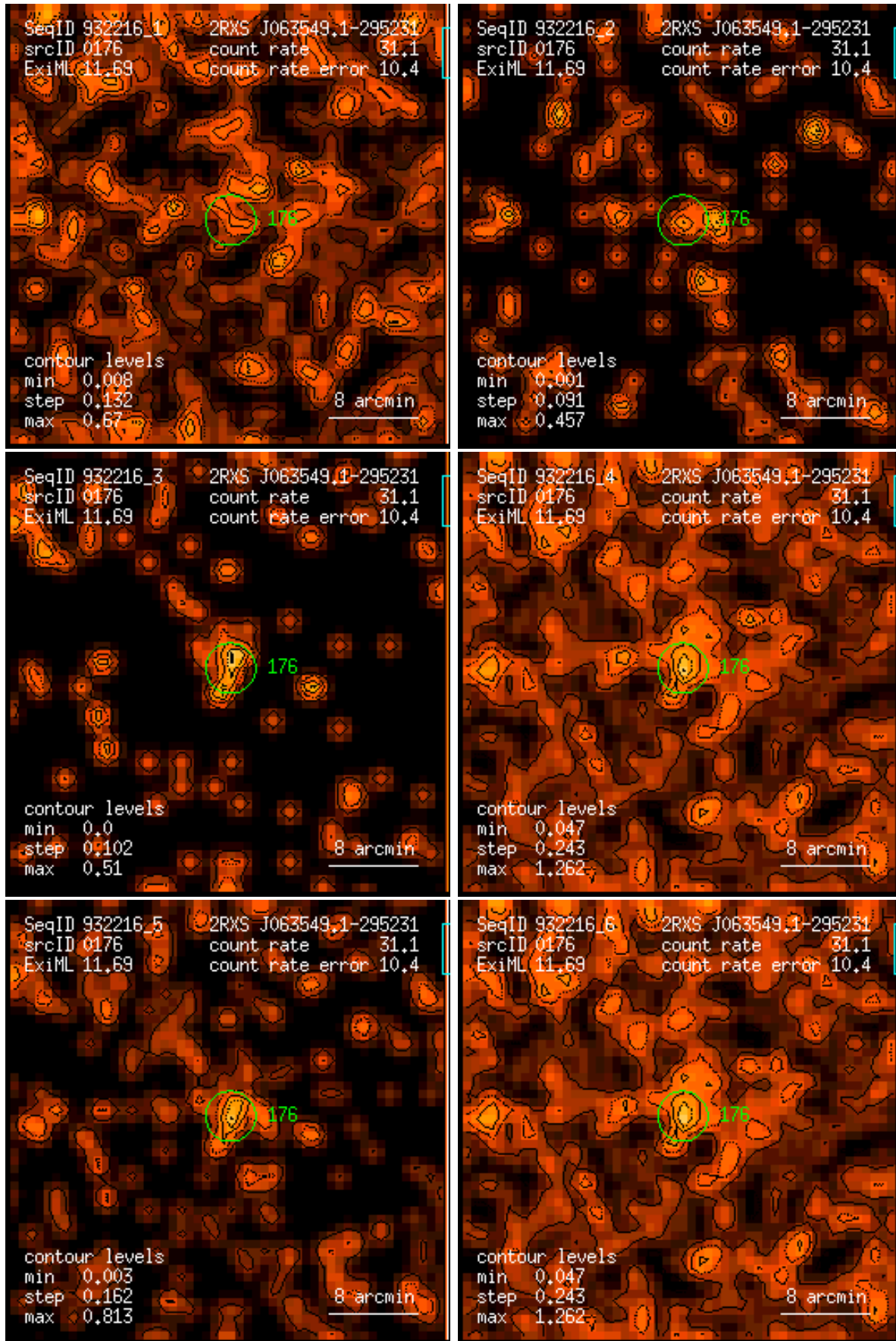
Figure 176: RASS 932216: detection 0176: band rate images, Gaussian filter: (1) PSPC channels 11 – 41, (2) 52 – 90, (3) 91 – 201, (4) 11 – 235, (5) 52 – 201, (6) 11 – 201. Broad band rates in counts/ks. Band rate contour levels in counts/ks/arcmin 2 .
