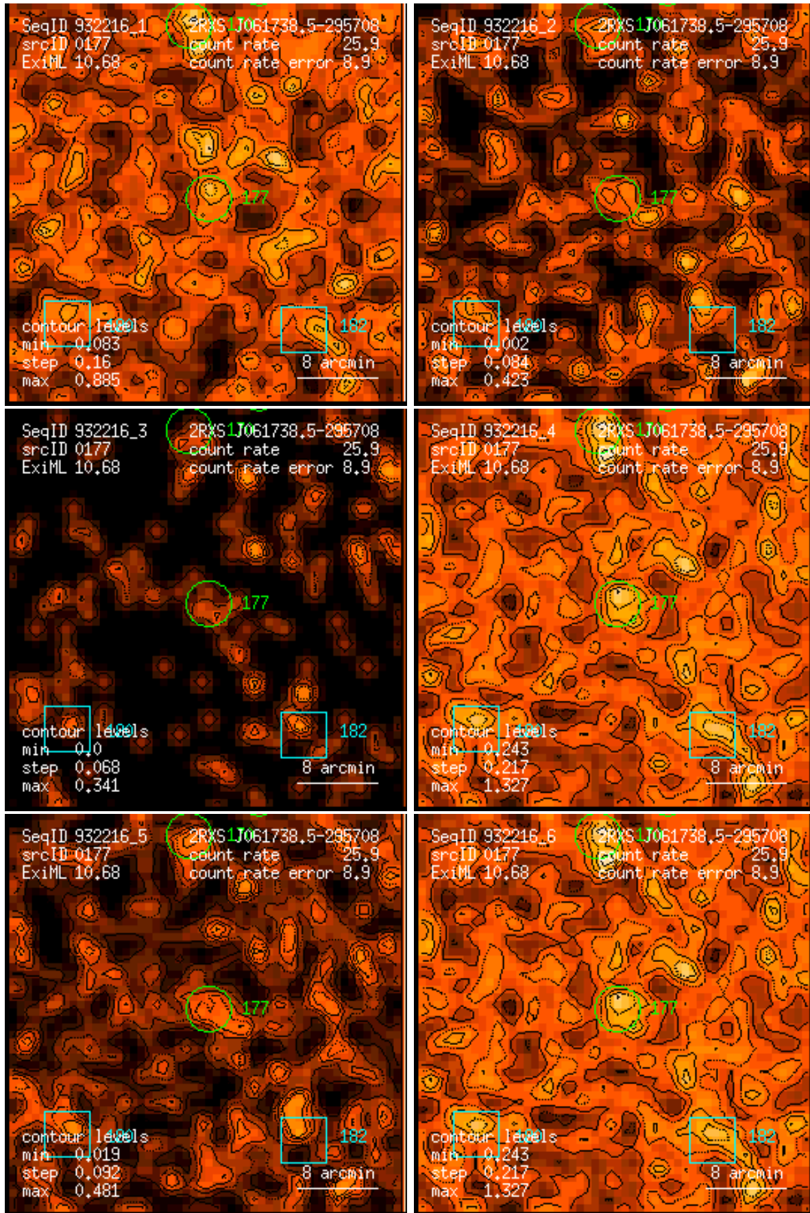
Figure 177: RASS 932216: detection 0177: band rate images, Gaussian filter: (1) PSPC channels 11 – 41, (2) 52 – 90, (3) 91 – 201, (4) 11 – 235, (5) 52 – 201, (6) 11 – 201. Broad band rates in counts/ks. Band rate contour levels in counts/ks/arcmin 2 .
