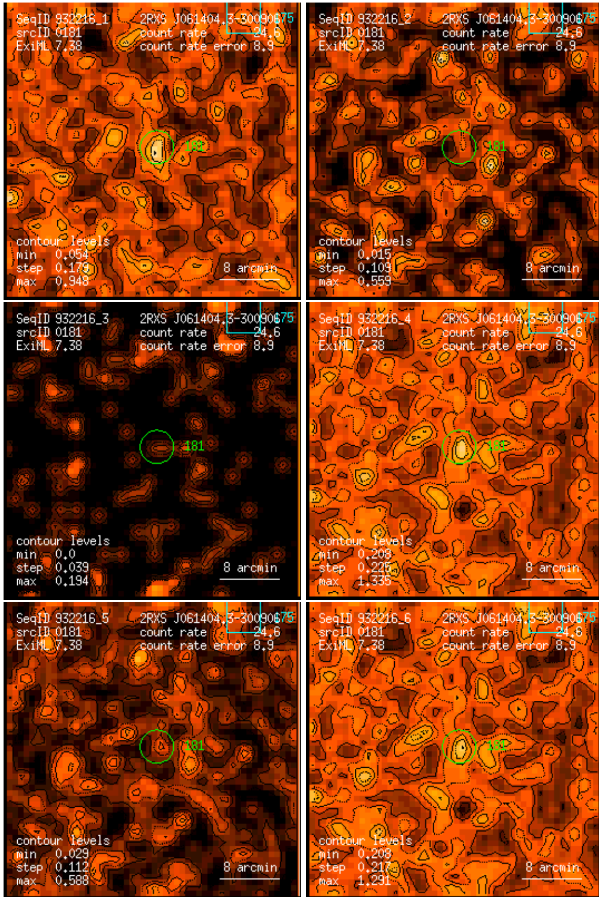
Figure 181: RASS 932216: detection 0181: band rate images, Gaussian filter: (1) PSPC channels 11 – 41, (2) 52 – 90, (3) 91 – 201, (4) 11 – 235, (5) 52 – 201, (6) 11 – 201. Broad band rates in counts/ks. Band rate contour levels in counts/ks/arcmin 2 .
