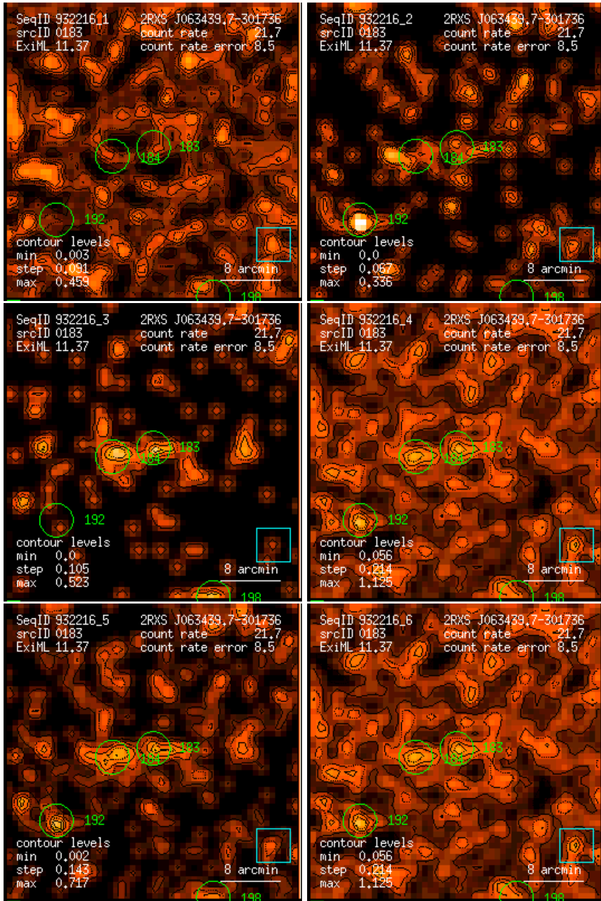
Figure 183: RASS 932216: detection 0183: band rate images, Gaussian filter: (1) PSPC channels 11 – 41, (2) 52 – 90, (3) 91 – 201, (4) 11 – 235, (5) 52 – 201, (6) 11 – 201. Broad band rates in counts/ks. Band rate contour levels in counts/ks/arcmin 2 .
