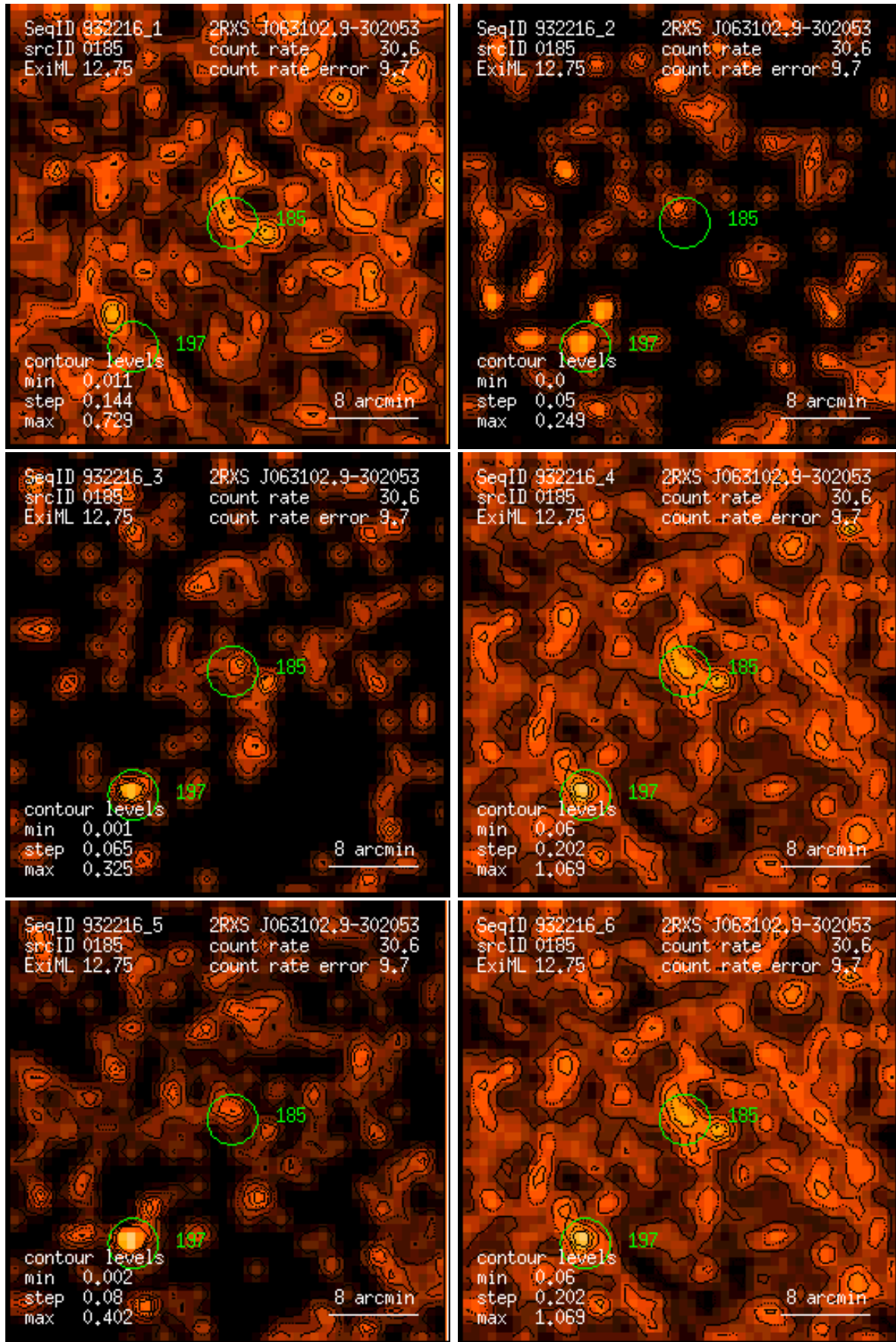
Figure 185: RASS 932216: detection 0185: band rate images, Gaussian filter: (1) PSPC channels 11 – 41, (2) 52 – 90, (3) 91 – 201, (4) 11 – 235, (5) 52 – 201, (6) 11 – 201. Broad band rates in counts/ks. Band rate contour levels in counts/ks/arcmin 2 .
