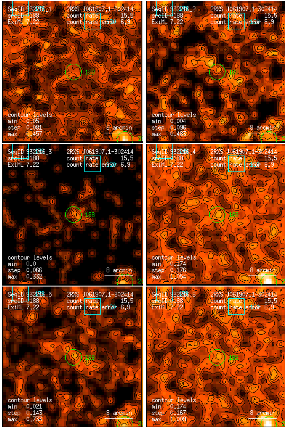
Figure 188: RASS 932216: detection 0188: band rate images, Gaussian filter: (1) PSPC channels 11 – 41, (2) 52 – 90, (3) 91 – 201, (4) 11 – 235, (5) 52 – 201, (6) 11 – 201. Broad band rates in counts/ks. Band rate contour levels in counts/ks/arcmin 2 .
