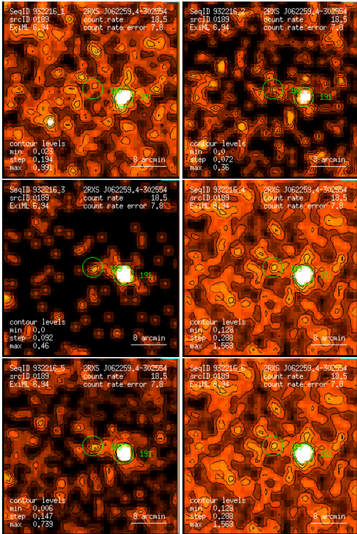
Figure 189: RASS 932216: detection 0189: band rate images, Gaussian filter: (1) PSPC channels 11 – 41, (2) 52 – 90, (3) 91 – 201, (4) 11 – 235, (5) 52 – 201, (6) 11 – 201. Broad band rates in counts/ks. Band rate contour levels in counts/ks/arcmin 2 .
