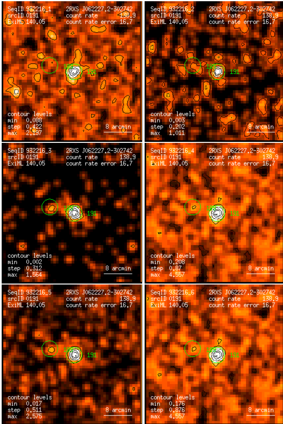
Figure 191: RASS 932216: detection 0191: band rate images, Gaussian filter: (1) PSPC channels 11 – 41, (2) 52 – 90, (3) 91 – 201, (4) 11 – 235, (5) 52 – 201, (6) 11 – 201. Broad band rates in counts/ks. Band rate contour levels in counts/ks/arcmin 2 .
