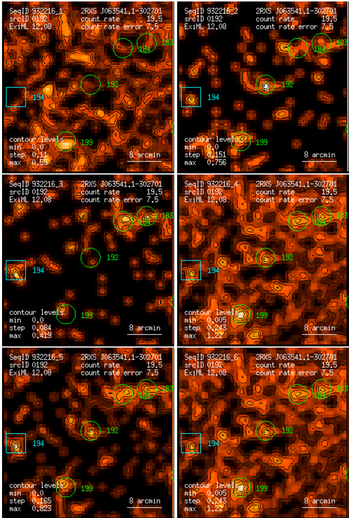
Figure 192: RASS 932216: detection 0192: band rate images, Gaussian filter: (1) PSPC channels 11 – 41, (2) 52 – 90, (3) 91 – 201, (4) 11 – 235, (5) 52 – 201, (6) 11 – 201. Broad band rates in counts/ks. Band rate contour levels in counts/ks/arcmin 2 .
