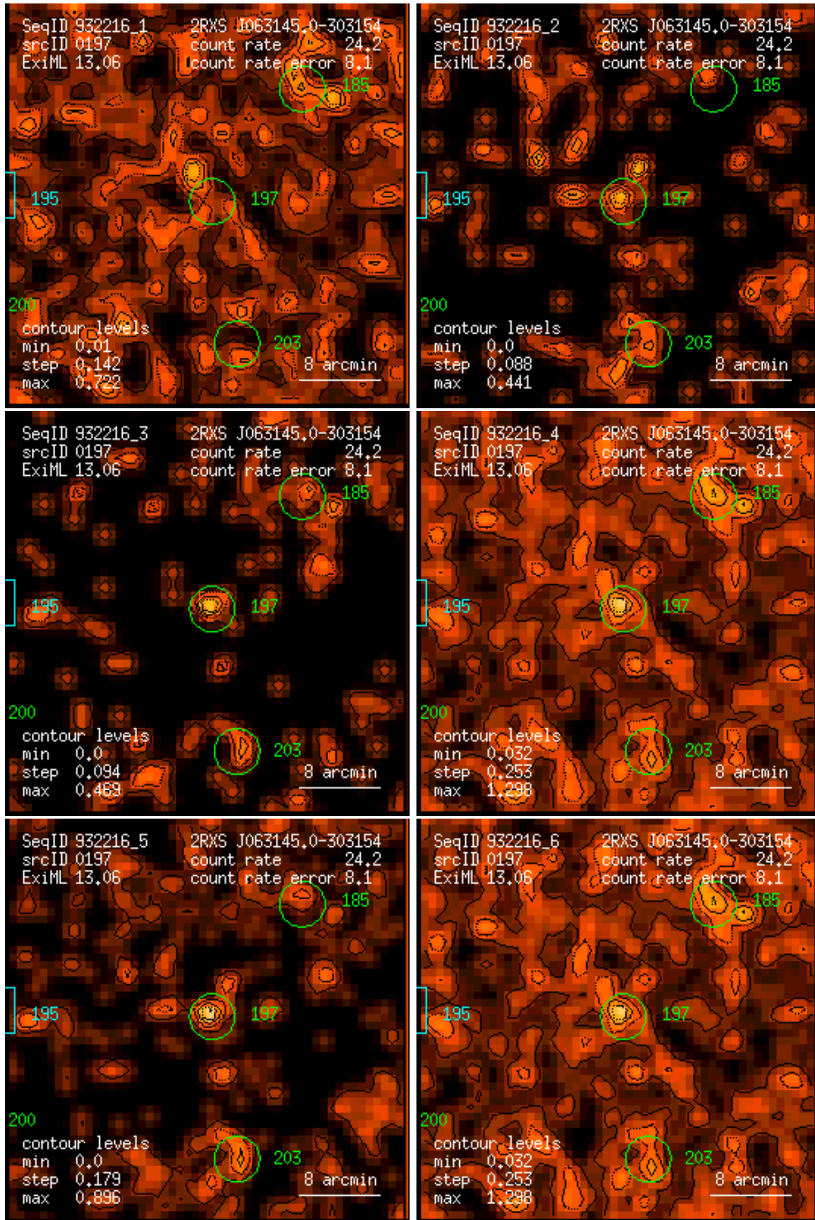
Figure 197: RASS 932216: detection 0197: band rate images, Gaussian filter: (1) PSPC channels 11 – 41, (2) 52 – 90, (3) 91 – 201, (4) 11 – 235, (5) 52 – 201, (6) 11 – 201. Broad band rates in counts/ks. Band rate contour levels in counts/ks/arcmin 2 .
