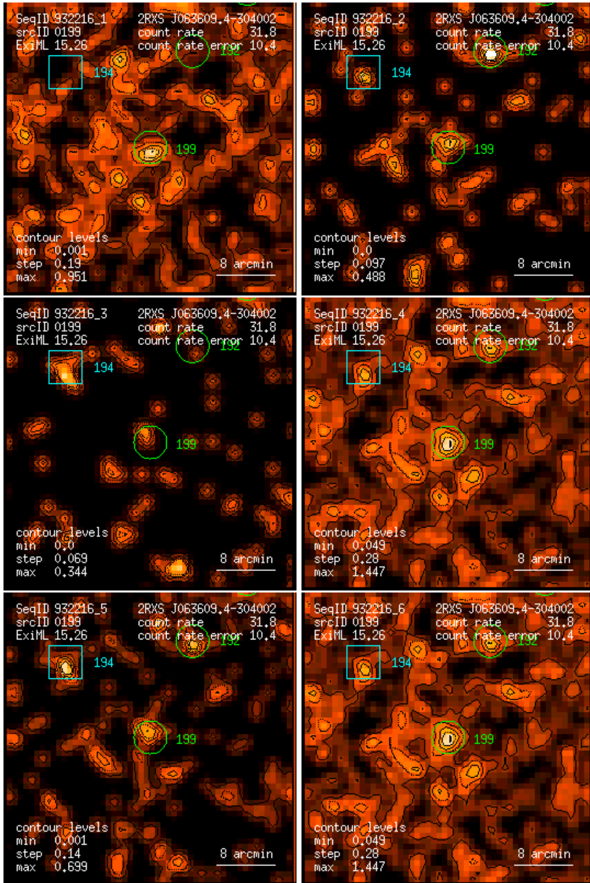
Figure 199: RASS 932216: detection 0199: band rate images, Gaussian filter: (1) PSPC channels 11 – 41, (2) 52 – 90, (3) 91 – 201, (4) 11 – 235, (5) 52 – 201, (6) 11 – 201. Broad band rates in counts/ks. Band rate contour levels in counts/ks/arcmin 2 .
