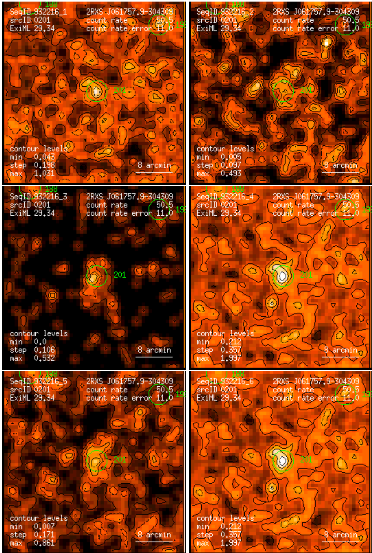
Figure 201: RASS 932216: detection 0201: band rate images, Gaussian filter: (1) PSPC channels 11 – 41, (2) 52 – 90, (3) 91 – 201, (4) 11 – 235, (5) 52 – 201, (6) 11 – 201. Broad band rates in counts/ks. Band rate contour levels in counts/ks/arcmin 2 .
