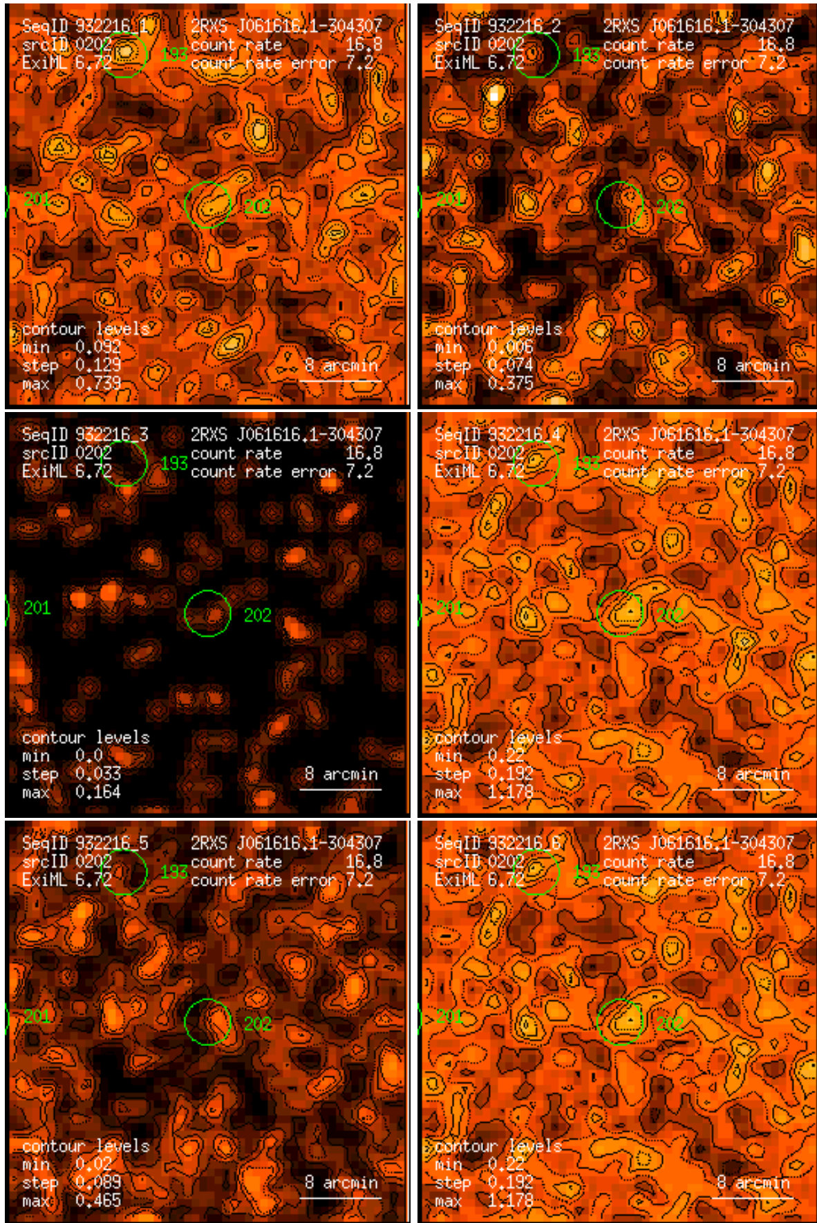
Figure 202: RASS 932216: detection 0202: band rate images, Gaussian filter: (1) PSPC channels 11 – 41, (2) 52 – 90, (3) 91 – 201, (4) 11 – 235, (5) 52 – 201, (6) 11 – 201. Broad band rates in counts/ks. Band rate contour levels in counts/ks/arcmin 2 .
