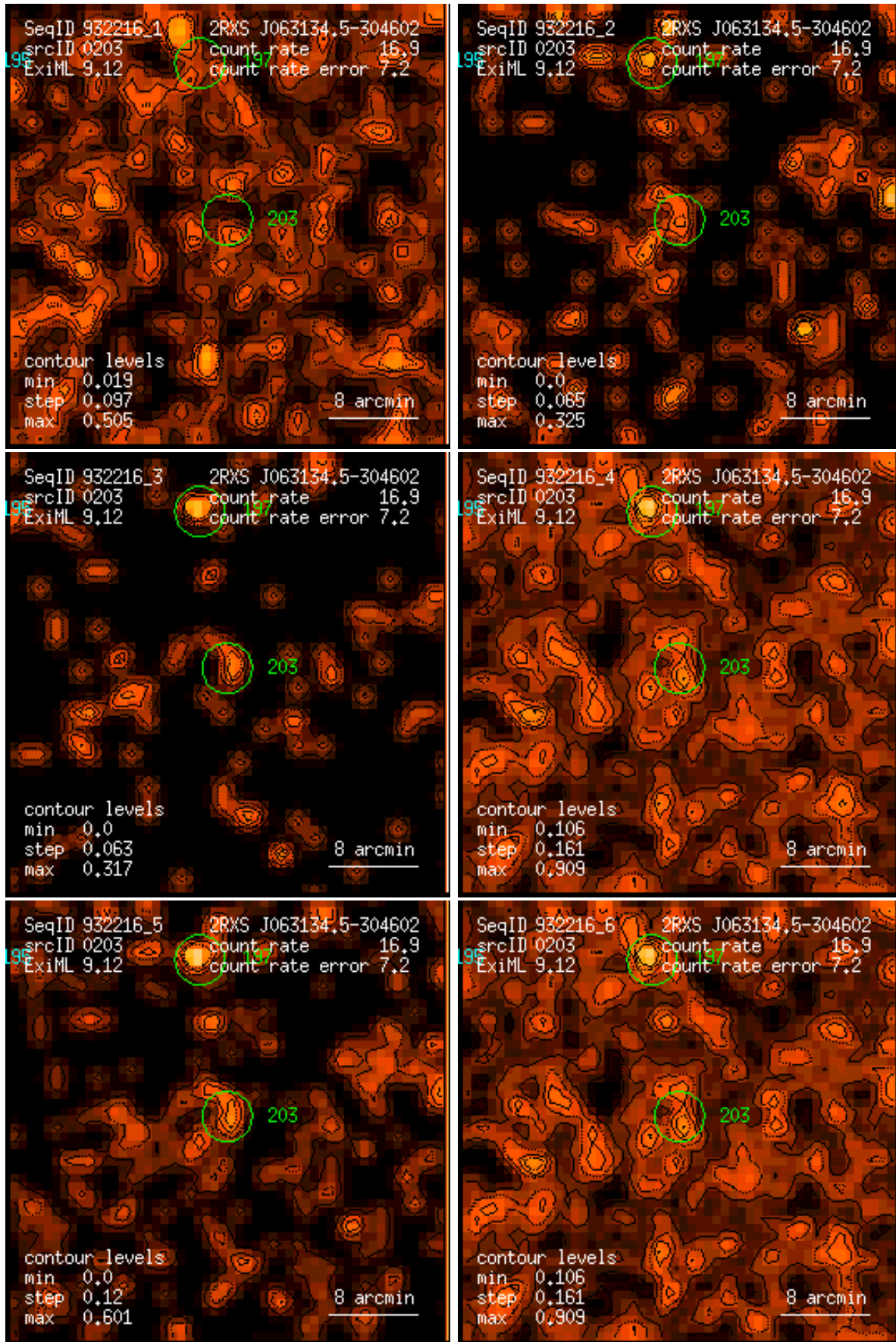
Figure 203: RASS 932216: detection 0203: band rate images, Gaussian filter: (1) PSPC channels 11 – 41, (2) 52 – 90, (3) 91 – 201, (4) 11 – 235, (5) 52 – 201, (6) 11 – 201. Broad band rates in counts/ks. Band rate contour levels in counts/ks/arcmin 2 .
