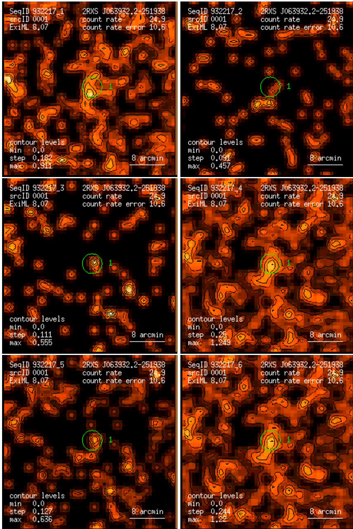
Figure 1: RASS 932217: detection 0001: band rate images, Gaussian filter: (1) PSPC channels 11 – 41, (2) 52 – 90, (3) 91 – 201, (4) 11 – 235, (5) 52 – 201, (6) 11 – 201. Broad band rates in counts/ks. Band rate contour levels in counts/ks/arcmin 2 .
