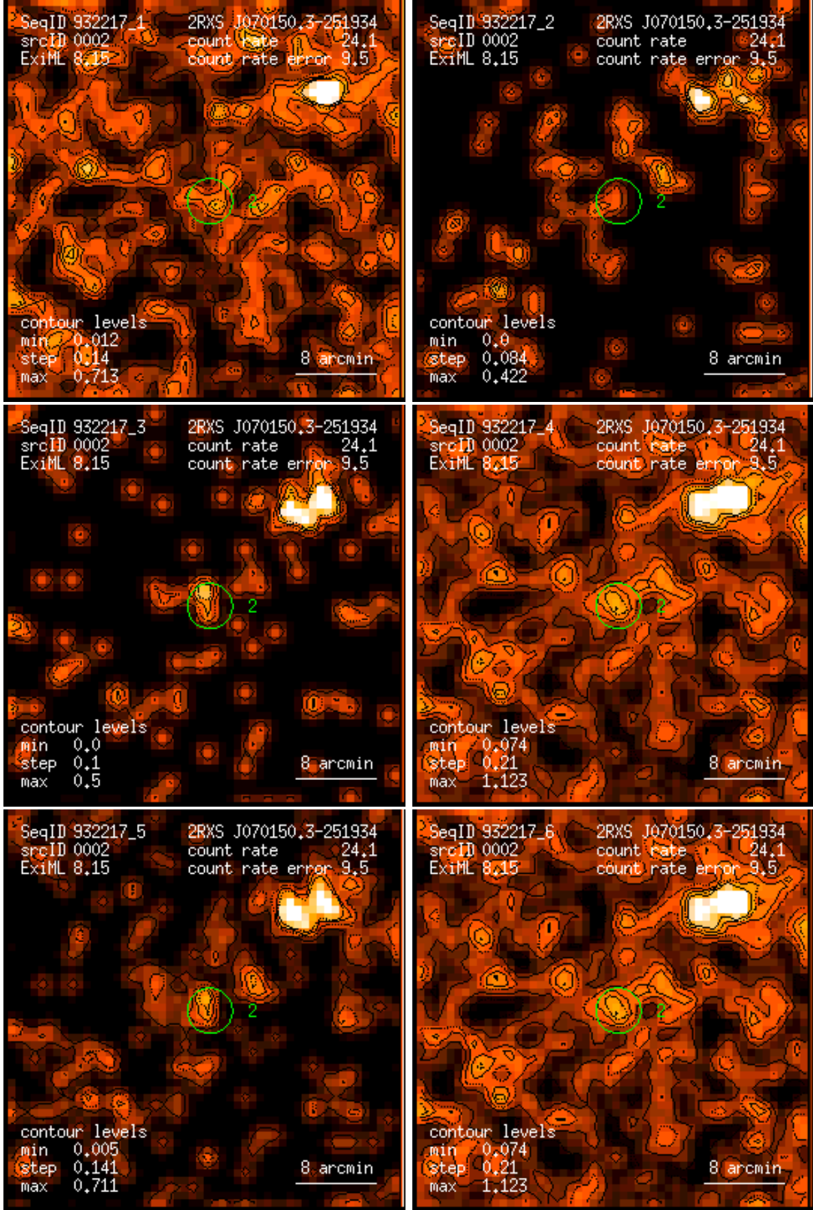
Figure 2: RASS 932217: detection 0002: band rate images, Gaussian filter: (1) PSPC channels 11 – 41, (2) 52 – 90, (3) 91 – 201, (4) 11 – 235, (5) 52 – 201, (6) 11 – 201. Broad band rates in counts/ks. Band rate contour levels in counts/ks/arcmin 2 .
